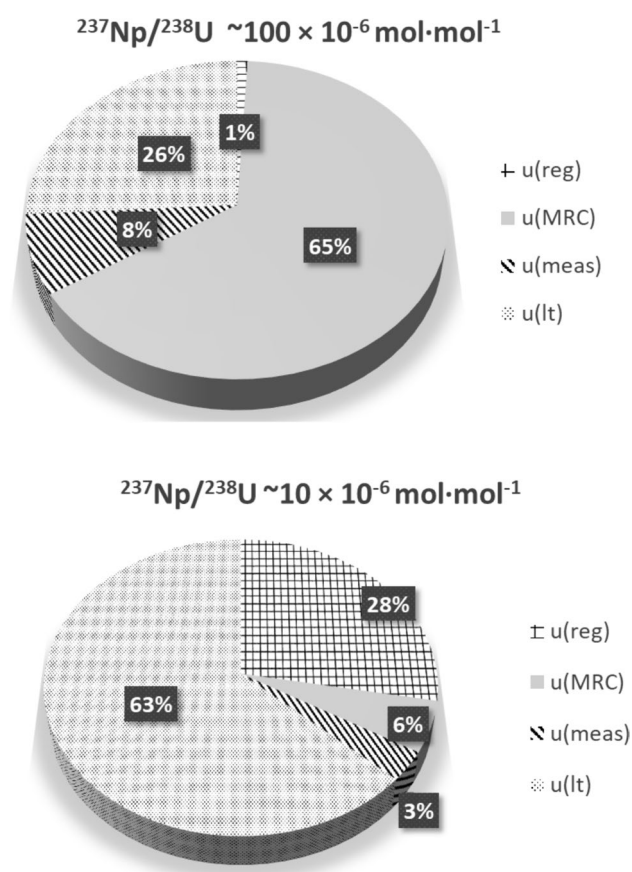
Fig. 6 Uncertainty budget on two samples: one with ^{237}\text{Np}/^{238}\text{U} = 10 \times 10^{-6} \text{ mol}\cdot\text{mol}^{-1} and one with ^{237}\text{Np}/^{238}\text{U} = 100 \times 10^{-6} \text{ mol}\cdot\text{mol}^{-1}
