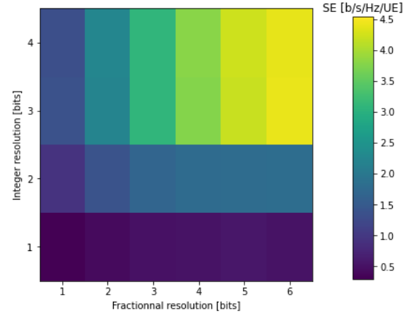
Fig. 4. Mediane per-UE SE against resolution of the DAC
