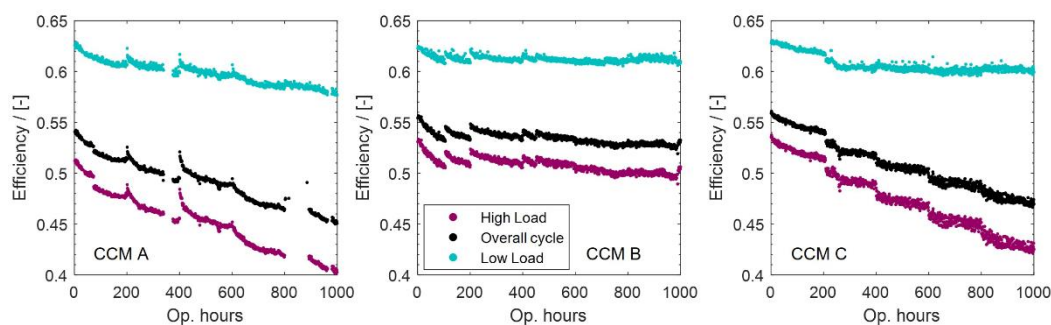
Figure 8 Cycle efficiency of each tested CCM evaluated as a function of operating hours. Efficiency is evaluated according to Equation 8. Overall cycle is compared against low load and high load operation, defined as included in the load cycle protocol section.
