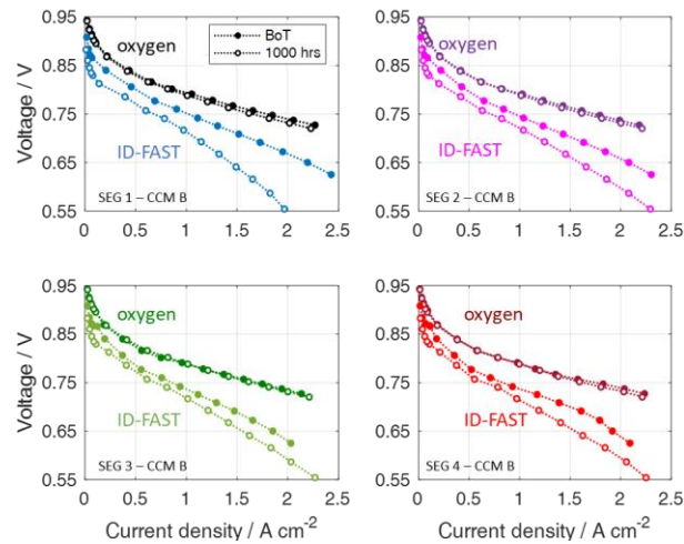
Figure 6 CCM B performance: oxygen and ID-FAST polarization curves (Table 2) are reported, in dark and light colours respectively. Local performance of each segment is compared at BoT (full dots) and after 1000 operating hours of load cycle protocol (empty dots).
