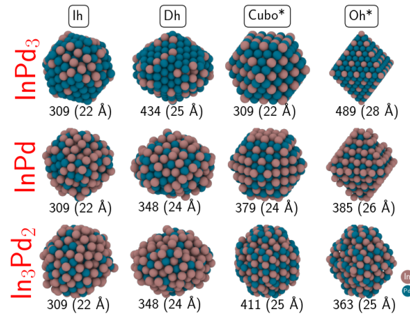
Fig. 4 Non-crystalline (Ih and Dh) and crystalline (Oh and Cubo) morphologies of \text{In}_3\text{Pd}_2 , \text{InPd} and \text{InPd}_3 NPs. The diameter of each NP is given, along with its number of atoms. Colour code: Pd = blue and In = brown.
