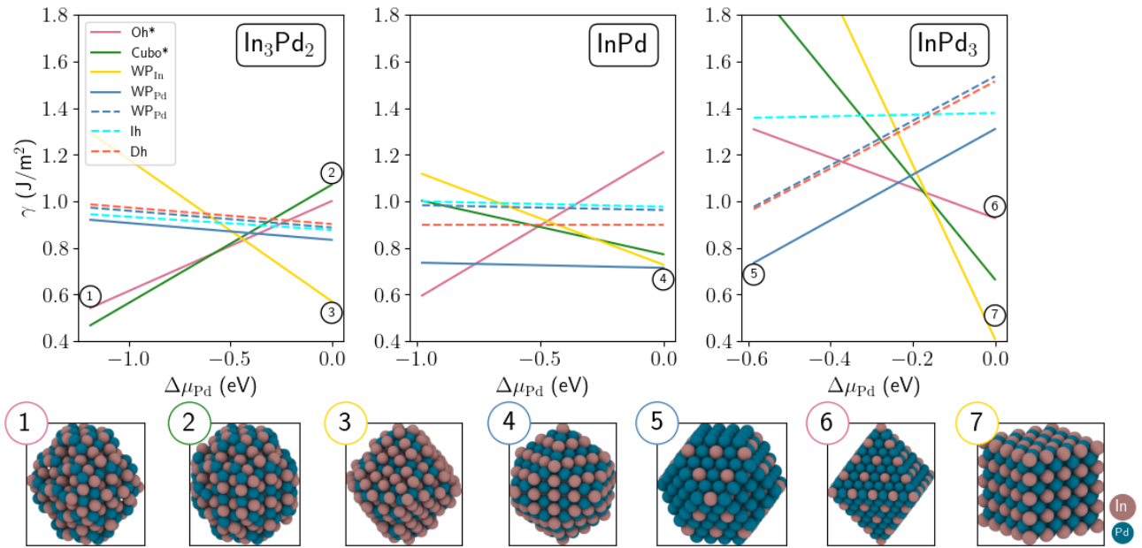
Fig. 5 Surface energies of \text{In}_3\text{Pd}_2 (left), \text{InPd} (middle) and \text{InPd}_3 (right) NPs as a function of \Delta\mu_{\text{Pd}} = \mu_{\text{Pd}} - \mu_{\text{Pd}}^b . Chemically ordered and disordered NPs are shown with full and dashed lines, respectively. Colour code: Pd = blue and In = brown.
