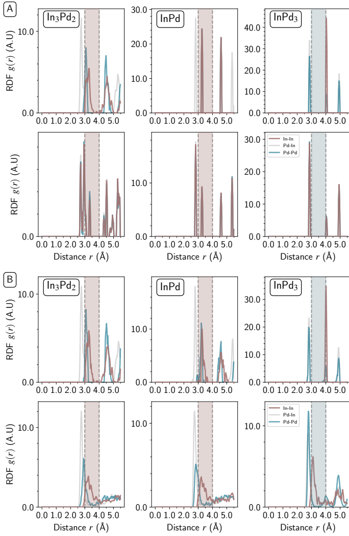
Fig. 9 Radial distribution function of In-In (brown), Pd-Pd (blue) and In-Pd (grey) bounds for small Pd-rich Wulff Polyhedra nanoparticles (diameter 24 Å) of \text{In}_3\text{Pd}_2 (left), \text{InPd} (middle), \text{InPd}_3 (right) compounds. The upper row displays ordered \text{WPd} whereas the bottom row represents disordered \text{WPd} . Radial function distributions for non relaxed and relaxed nanoparticles are drawn in figure A (top) and B (bottom), respectively. Blue filled area represents the attractive domain of In-In interactions in \text{InPd}_3 NPs. Red filled areas represent the repulsive domain of In-In interactions in \text{In}_3\text{Pd}_2 and \text{InPd} NPs. ( \mathcal{S} = [3.0 \text{ \AA}, 4.0 \text{ \AA}] )
