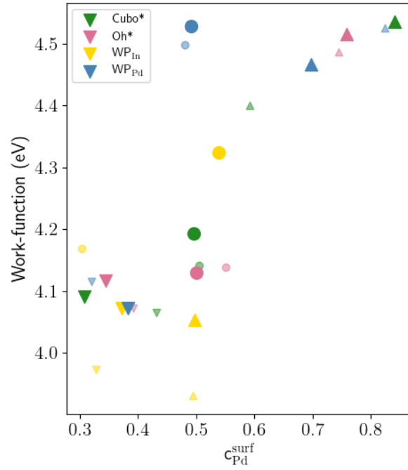
Fig. 11 Work-function (in eV) as a function of the surface Pd concentration (in at. %). Small and large symbols correspond to small and large nanoparticles, respectively. Colours give the NP morphologies while symbols give the compound ( \nabla In 3 Pd 2 , \circ InPd, \triangle InPd 3 ) from which it has been built. Data are gathered in Tab. S4.
