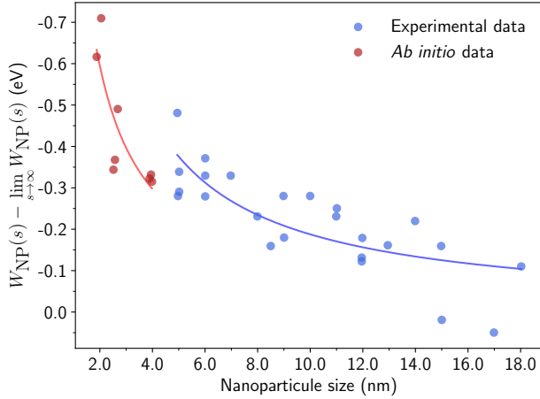
Fig. 10 Direct comparison between computed and measured work-function for gold NPs. Experimental data (in blue) are extracted from Ref. 100 and ab initio work-functions (in red) are calculated based on our methodology.
