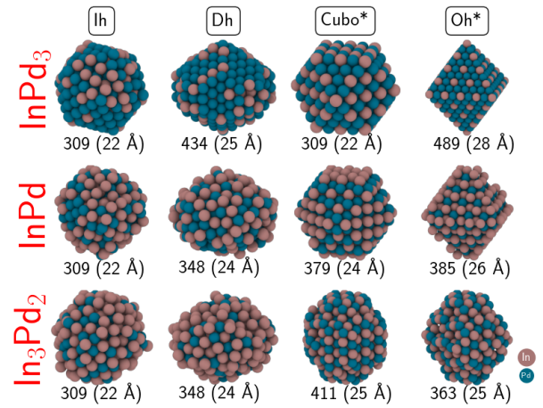
Fig. 4 Non-crystalline (Ih and Dh) and crystalline (Oh and Cubo) morphologies of \text{In}_3\text{Pd}_2 , \text{InPd} and \text{InPd}_3 NPs. The diameter of each NP is given, along with its number of atoms. Colour code: Pd = blue and In = brown.
