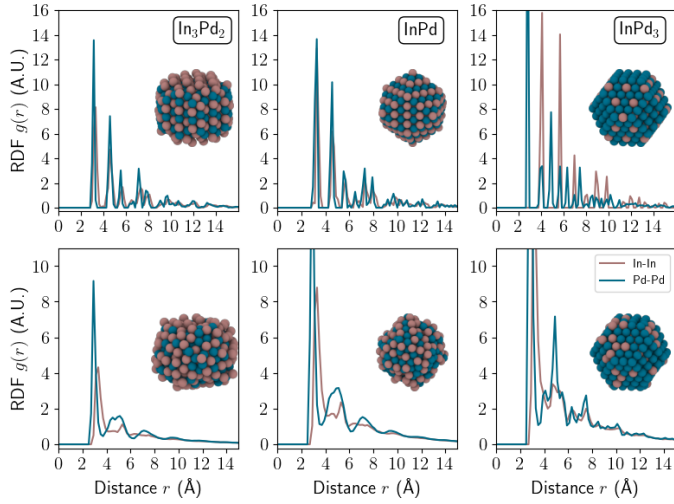
Fig. 6 Radial distribution function of In-In (brown) and Pd-Pd (blue) bonds as a function of the distance from the NP centre ( r ). The considered NPs are small WP Pd nanoparticles (diameter 24 Å) of In 3 Pd 2 (left), InPd (middle), InPd 3 (right) compounds. The upper and bottom rows correspond to ordered and disordered WP Pd NPs, respectively. Colour code: Pd = blue and In = brown.
