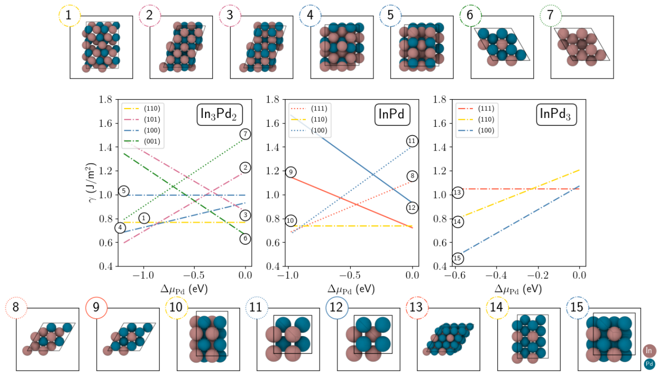
Fig. 2 Surface energies of \text{In}_3\text{Pd}_2(hkl) (left), \text{InPd}(hkl) (middle) and \text{InPd}_3(hkl) (right) as a function of \Delta\mu_{\text{Pd}} = \mu_{\text{Pd}} - \mu_{\text{Pd}}^{\text{b}} where \mu_{\text{Pd}} is the chemical potential of Pd in the compound and \mu_{\text{Pd}}^{\text{b}} is the cohesive energy of elemental Pd bulk. Pure Pd, pure In and mixed terminations are shown with solid, dashed and dash-dotted lines, respectively. Only the most stable surfaces are represented. Colour code for surface terminations: Pd = blue and In = brown.
