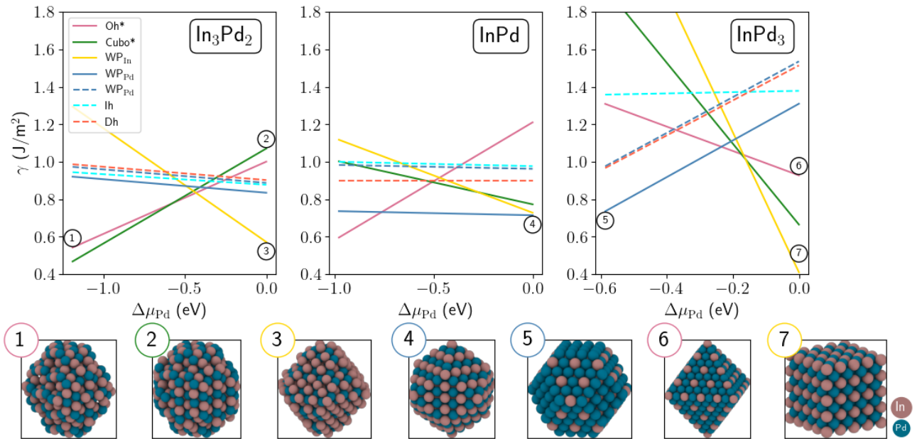
Fig. 5 Surface energies of \text{In}_3\text{Pd}_2 (left), \text{InPd} (middle) and \text{InPd}_3 (right) NPs as a function of \Delta\mu_{\text{Pd}} = \mu_{\text{Pd}} - \mu_{\text{Pd}}^{\text{b}} . Chemically ordered and disordered NPs are shown with full and dashed lines, respectively. Colour code: Pd = blue and In = brown.
