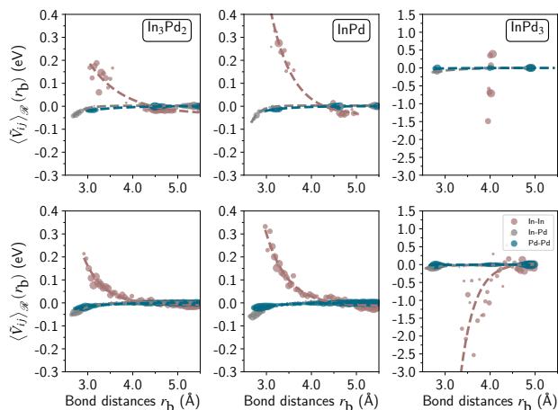
Fig. 8 Radial average \bar{V}_{ij} energy ( \langle\bar{V}_{ij}\rangle(r_b) ) of In-In bonds (brown), Pd-Pd bonds (blue) and In-Pd bonds (grey) for small NPs (diameter 24 Å) built by the Wulff construction using \text{In}_3\text{Pd}_2 (left), \text{InPd} (middle), \text{InPd}_3 (right) bulk compounds. The upper and bottom rows display ordered and disordered \text{WP}_{\text{Pd}} , respectively. Dots are brute data and dashed lines result from interpolation. Dot sizes are proportional to bond numbers.
