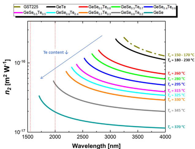
Figure 4. Nonlinear Kerr ( n_2 ) refractive index as a function of wavelength for the amorphous as-deposited GeSe 1-x Te x thin films. The n_2 curves were obtained by means of Sheik-Bahae model (see text and references [33,34,38] ). In each case, the data were plotted only in the spectral range for which the TPA losses are limited (see text).
