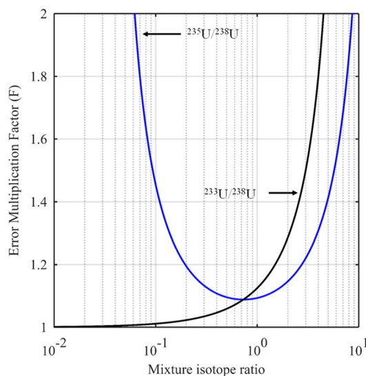
Fig. 2 Error multiplication factor as a function of the ^{235}\text{U}/^{238}\text{U} mixture isotope ratio (blue curve) for a sample with ^{235}\text{U}/^{238}\text{U} = 0.0309 and for a spike enriched with the ^{235}\text{U} isotope ( ^{235}\text{U}/^{238}\text{U} = 17.3 ), and as a function of the ^{233}\text{U}/^{238}\text{U} mixture isotope ratio (black curve) for a sample with ^{233}\text{U}/^{238}\text{U} = 0 and for a spike enriched with a ^{233}\text{U} isotope ( ^{233}\text{U}/^{238}\text{U} = 9 ).
