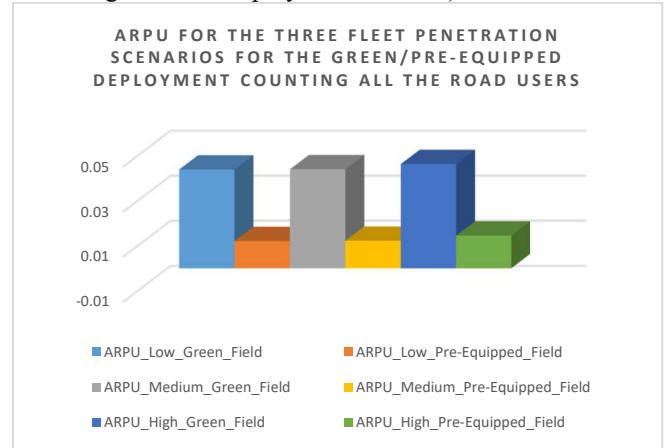
Figure 8 : ARPU for the three fleet penetration scenarios for the green/pre-equipped deployment counting all the road users
