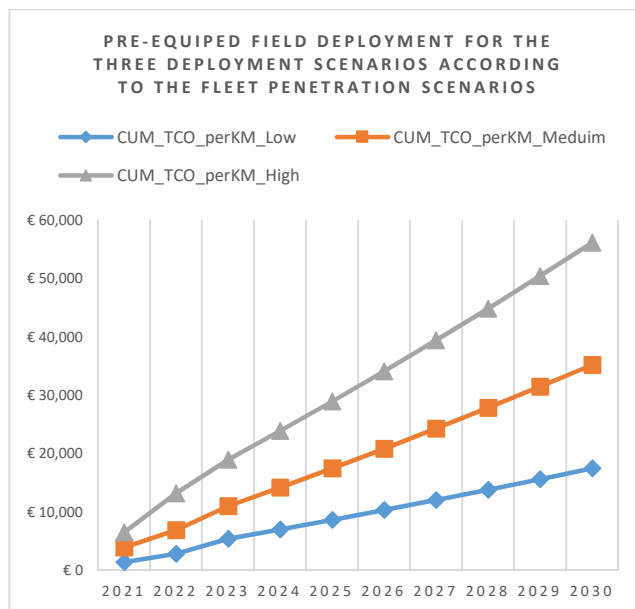
Figure 2: Cumulative TCO per km for the low, medium, and high deployment scenarios for a pre-equipped field corridor segment
