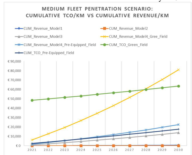
Figure 4: Medium fleet penetration scenario: Cumulative TCO/km VS Cumulative Revenue/km for the four revenue models
