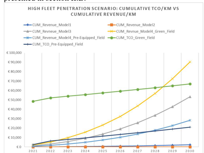
Figure 5: High fleet penetration scenario: Cumulative TCO/km VS Cumulative Revenue/km for the four revenue models
