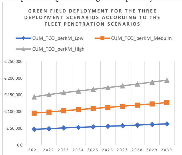
Figure 1: Cumulative TCO per km for the low, medium, and high deployment scenarios for a green field corridor segment
