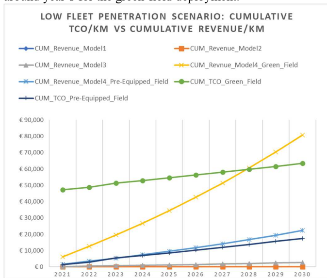
Figure 3: Low fleet penetration scenario: Cumulative TCO/km VS Cumulative Revenue/km for the four revenue models
