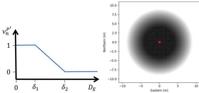
Fig. 3. Left: membership function for the “Near” relation. Right: corresponding structuring element \nu_n with \delta_1 = 4 and \delta_2 = 9
