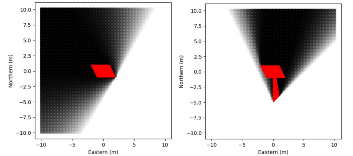
Fig. 2. Fuzzy landscape of two objects (crisp in this example) dilated by \nu_G . Set of parameters are as follow: left picture G = 300^\circ , \theta_1 = \pi/12 and \theta_2 = \pi/2 ; right picture G = 10^\circ , \theta_1 = 0 and \theta_2 = \pi/5
