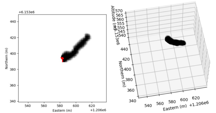
Fig. 8. Two-dimensional from above (left) and three-dimensional (right) representations of the same runoff area
