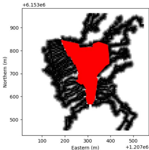
Fig. 11. Runoff area from the Corte castle
