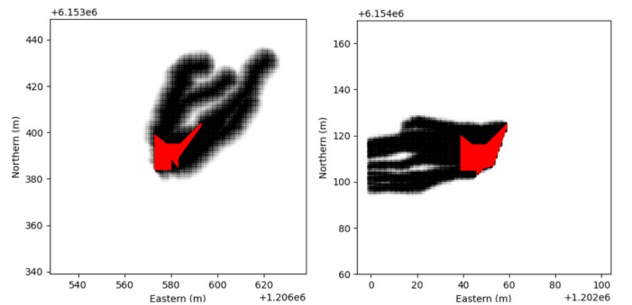
Fig. 9. Examples of runoff from crisper polygons, with various shapes and from different points on the DTM
