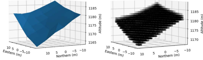
Fig. 7. Left: 20m \times 20m excerpt of the DTM. Right: Fuzzy set for the spatial relation “At Ground Level” on the same DTM area. Centered on E = 1201690 , N = 6147769 , for the sake of the example
