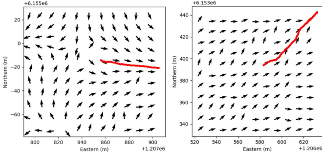
Fig. 5. Two fields of lines of greatest dip, with the line of greatest dip showing a runoff from the centre of the field is shown in red.
