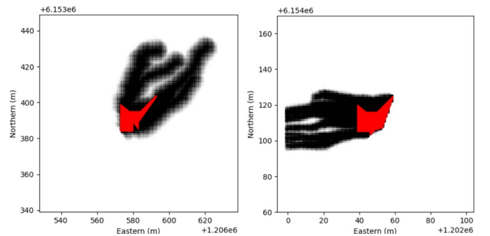
Fig. 9. Examples of runoff from craps polygons, with various shapes and from different points on the DTM
