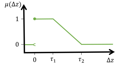
Fig. 6. Membership function “at ground level” with respect of the computed value of \Delta z for any point X of \mathbb{R}^3
