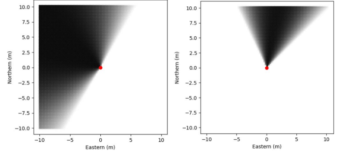
Fig. 1. Two structuring elements \nu_G representing the predicate “In the direction G ”. The red dot represents the centre of the structuring element. Set of parameters are as follow: left picture G = 300^\circ , \theta_1 = \pi/12 and \theta_2 = \pi/2 ; right picture G = 10^\circ , \theta_1 = 0 and \theta_2 = \pi/5
