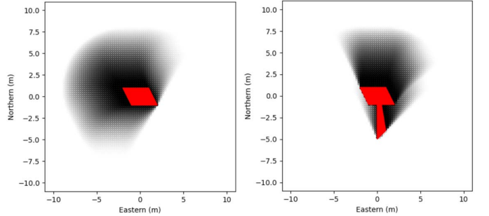
Fig. 4. The same objects of Figure 2 dilated by \nu_{NG} with the same sets of parameters, adding \delta_1 = 2 and \delta_2 = 7 for both pictures, considered in the plane of interest ( z = 0 )
