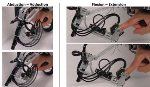
Figure 15: Hand movements for the force feedback tests.
