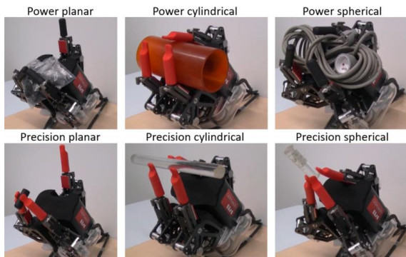
Figure 2: Illustration of the possible grasps of the CEA LIST's three fingers slave hand.
