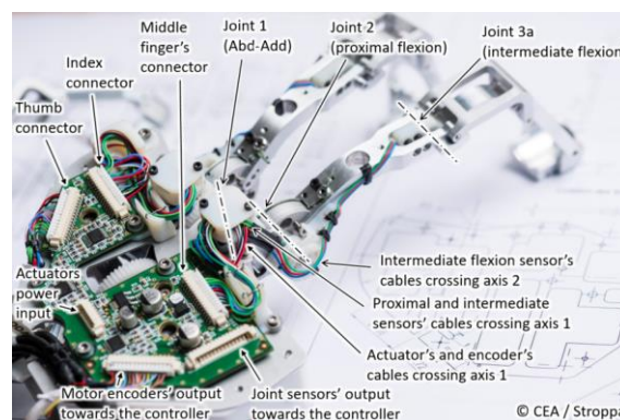
Figure 14: Dexterous hand master internal cabling.
