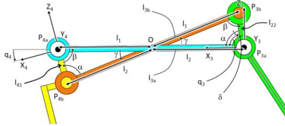
Figure 10: Inverted parallelogram.
