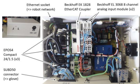
Figure 16: Dexterous hand master controller.
