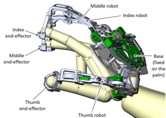
Figure 6: Overview of the tri-digital master glove.
