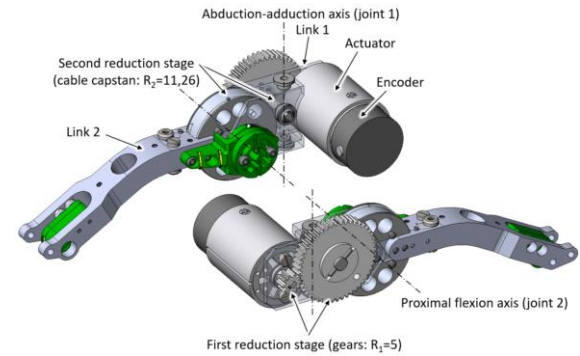
Figure 11: Actuation units.
