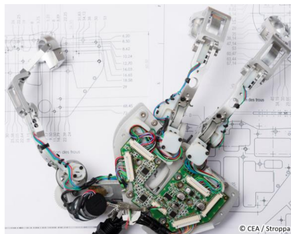
Figure 13: Internal view of the manufactured prototype of tri-digital dexterous hand master.
