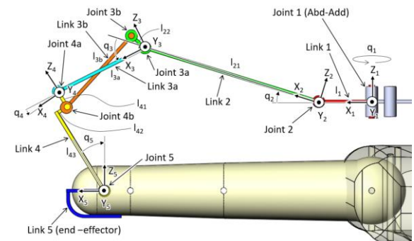
Figure 9: Kinematic model of the robots. A frame R_i=(O_i,X_i,Y_i,Z_i) is associated with each link, with its origin positioned on the joint axis, q_i is the rotation around joint i , and l_i (resp. l_{i1}, l_{i2} ) designates the length of link i (resp. of different parts of link i ).
