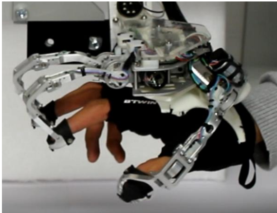
Figure 15: Fully integrated dexterous master glove.
