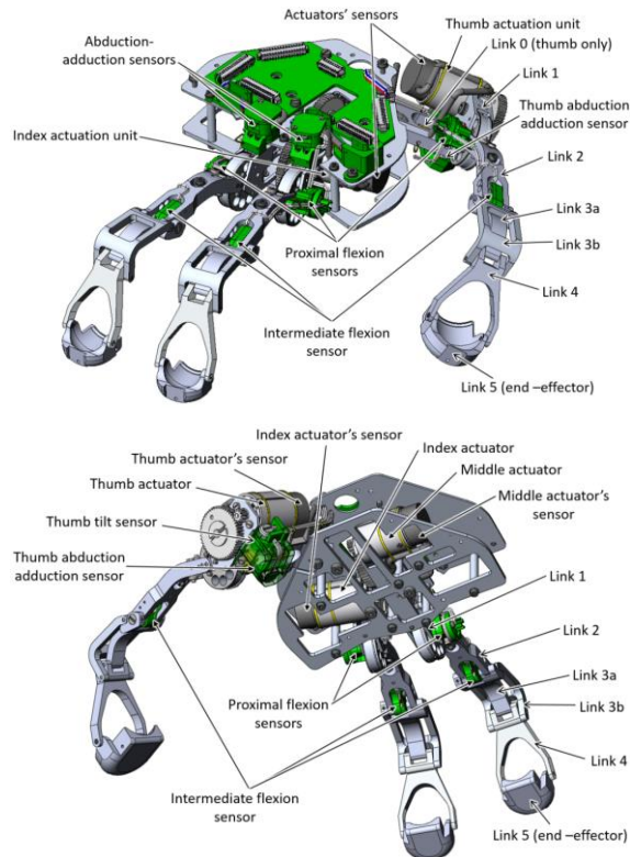
Figure 7: Main components of the master glove (top and bottom views).
