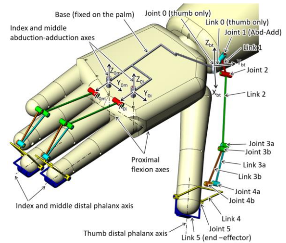
Figure 8: Kinematic model of the master glove ( R_{bt}=(O_{bt},X_{bt},Y_{bt},Z_{bt}) , resp. R_{0i}=(O_{0i},X_{0i},Y_{0i},Z_{0i}) and R_{0m}=(O_{0m},X_{0m},Y_{0m},Z_{0m}) are the base frames of the thumb, index and middle fingers).
