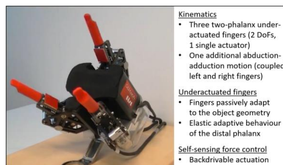
Figure 1: CEA LIST's three fingers slave hand.
