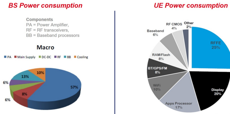
Figure 4.1: Power Consumption at BS and UE
