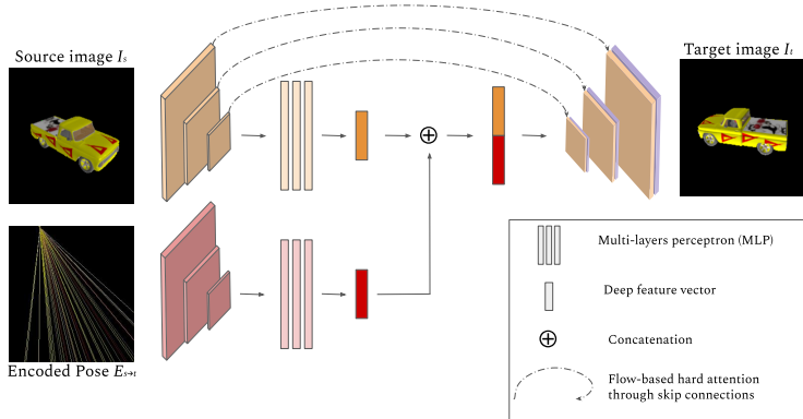
Figure 2: General overview of our architecture. Network takes as inputs both I_s and E_{s \rightarrow t} through two distinct encoders that produce feature vectors that are concatenated before being fed to the decoder. The network structure also leverage on the hard flow attention connections introduced in [9].
