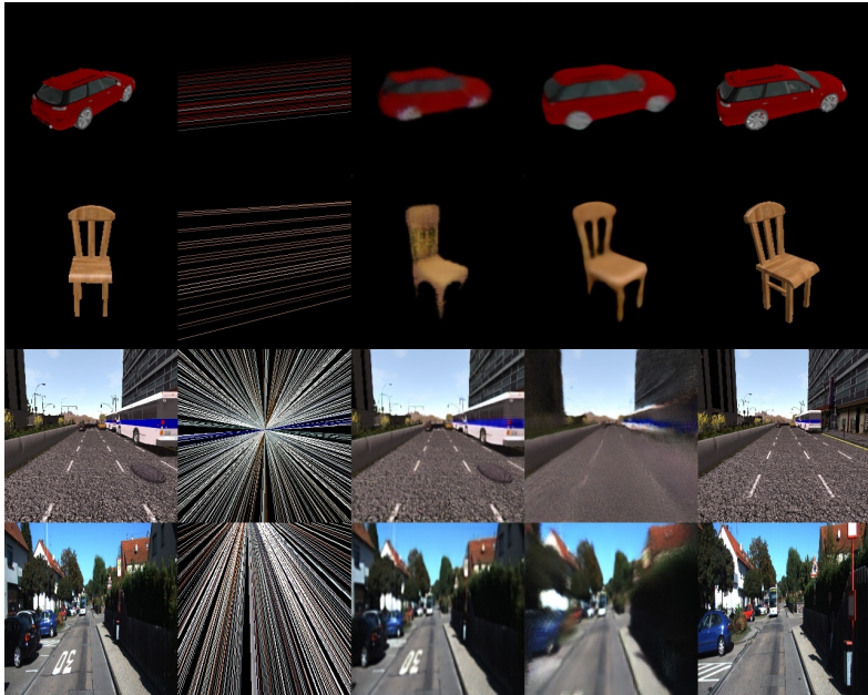
Figure 3: Inference results on all the four datasets considered. E_s \rightarrow_t encoded transformation have been obtained with \mathbf{G}_{15} . From left to right: the source image I_s , E_s \rightarrow_t , [9] prediction, our prediction, the target image I_t . On overall, our method predicts more consistent results since complete pose transformation has been fed to the network contrary to the concurrent work from [9].
