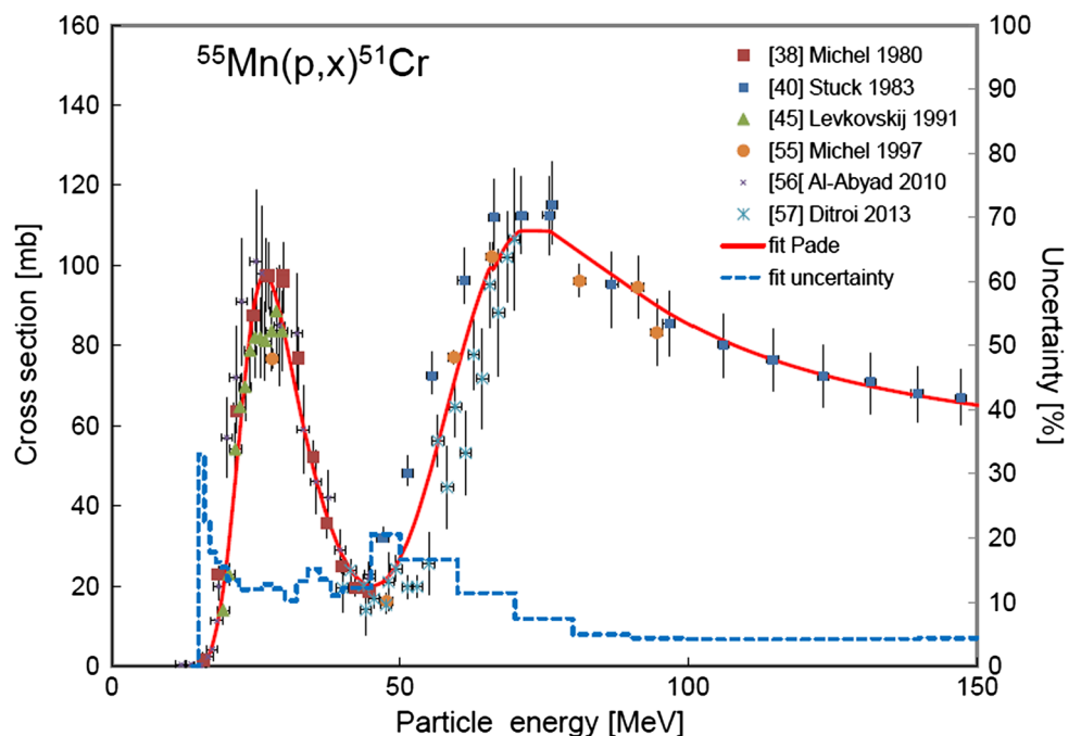
Fig. 6 Six experimental datasets for the ^{55}\text{Mn}(p,x)^{51}\text{Cr} reaction [38, 40, 45, 55–57] with the Padé fit ( L = 13 , N = 94 , \chi^2 = 1.75 ) and estimated uncertainties as percentages (dashed line, right-hand scale)
