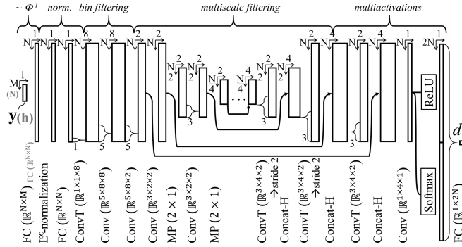
Fig. 4: Deep Generative Model topology for pixel-wise depth reconstruction. Note that the only difference between reconstruction from histogram inputs and from CS is the first Fully Connected (FC) layer. Concat-H corresponds to horizontal concatenation and MP corresponds to Max Pooling.
