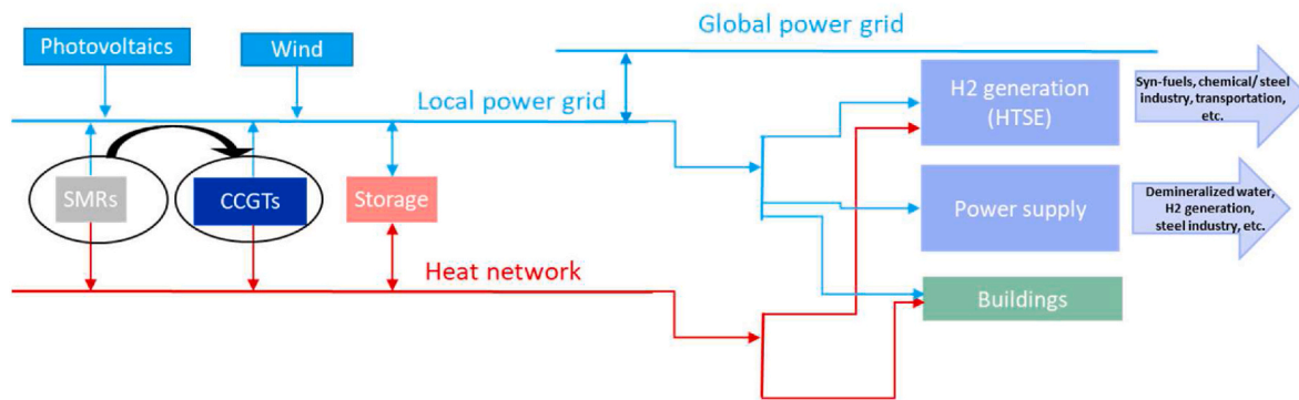
Fig. 5. Schematic configuration of the hybrid energy system corresponding to the energy hub.
