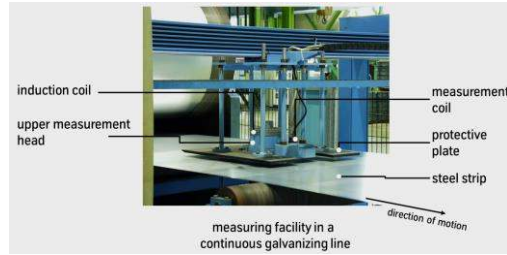
Figure 1: Set-up of the IMPOC measurement: the tested specimen is magnetised by means of two induction coils at its both sides and the remanent field is measured at the sensors location.
