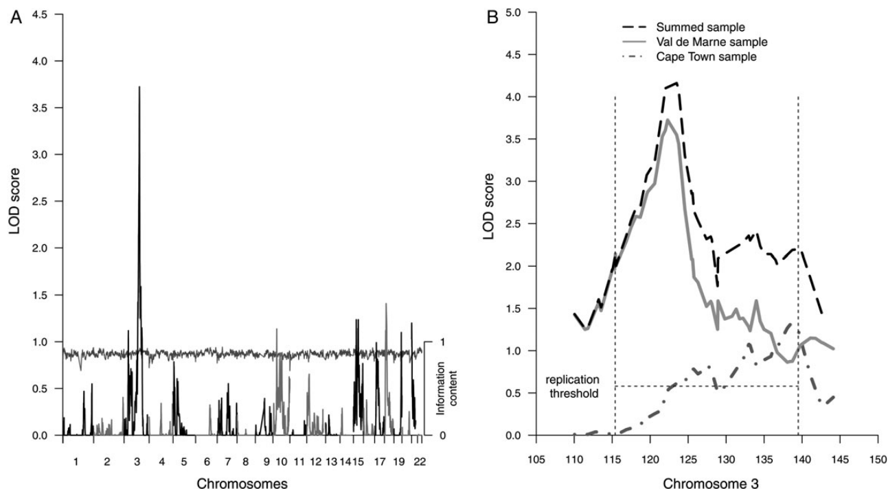
Figure 2. Model-free linkage analysis of the IFN \gamma -ESAT6 BCG phenotype described in Materials and Methods. A , Results for genome-wide analysis for the Val-de-Marne sample, showing multipoint LOD scores (left y-axis) and information content (horizontal line; right y-axis) for the 22 autosomes (x-axis). B , Expanded view of the linked chromosome 3 region from 105 to 150 Mb (x-axis). The multipoint LOD score is indicated on the y-axis for the Val-de-Marne sample (solid gray line), the Cape Town sample (double-dashed gray line), and the summed samples (black long-dash line). The horizontal dotted line indicates the significance threshold for replication, and the 2 vertical dotted lines delimit the confidence interval of the linked locus.
