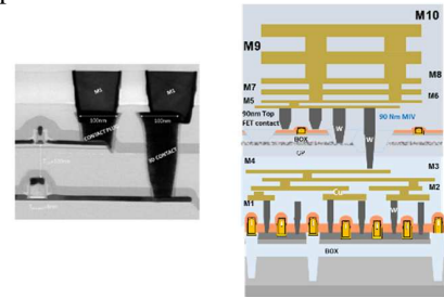
Fig. 5. Monolithic 3D : Cross section of silicon devices and BeOL
