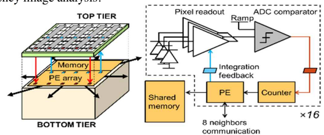
Fig. 8. Bloc diagram of the scalable Macropixel 3D structure
