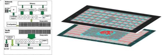
Fig. 11. 2 layer spiking neural network implemented into a 2 layer 3D-circuit
