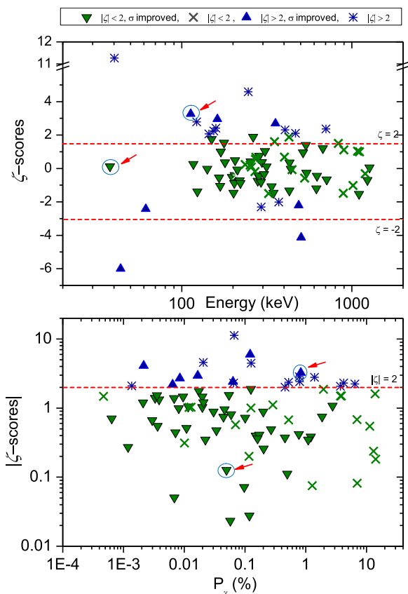
Fig. 7. Comparison of absolute \gamma -ray emission probabilities from this work with recommended data from the DDEP and the NDS databases using the \zeta -score. The circled data points indicate emission probabilities for which formerly no uncertainties were assigned.
