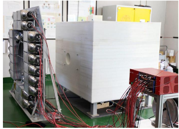
Fig. 5. Integration of the main components of C-BORD's RRTNIS at JRC Ispra, Italy.
