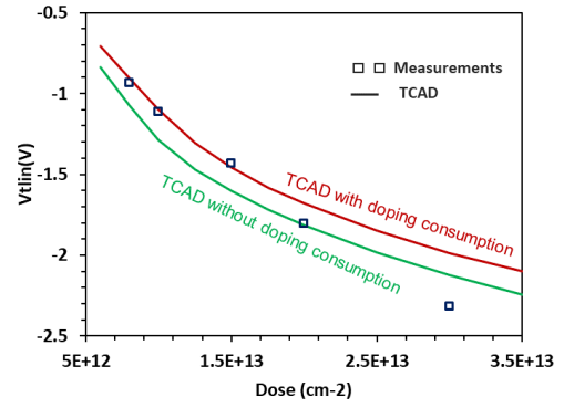
Fig. 8 : L=1\mu\text{m} V_{tlin} variation with Phosphorus implantation dose from measurement and TCAD
