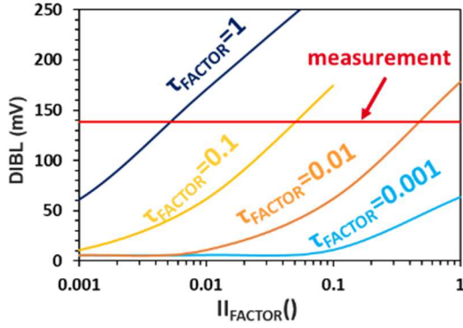
Fig. 13 : L=1\mu\text{m} DIBL variation with II_{\text{FACTOR}}(l) for several \tau_{\text{FACTOR}} at constant channel doping (Phosphorus dose 6.10^{12}\text{cm}^{-2} ) compare to measurement (red line)
