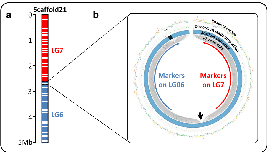
Fig. 2 Example of a clue leading to scaffold splitting. a Genetic markers mapped onto scaffold21 belong respectively to linkage-group 7 (red) and linkage-group 6 (blue) suggesting a chimeric misassembly. b CIRCOS graphical representation of paired read mapping in the misassembled region. This representation is drawn using Scaffremodler's tools. In the inner circle, links between read pairs are drawn with the following color code: grey lines correspond to concordant pairs (correct orientation and insert size), orange and red lines correspond to discordant pairs with smaller and greater insert size respectively. Purple lines correspond to pairs showing reverse-reverse orientation, green lines, forward-forward and blue lines correspond to pair with complete reverse orientation relative to the paired library construction. The second circle represents scaffold in blue with gaps as black regions. The next circles are scatter plots with warm-cool color code. The first scatter plot presents the proportion of discordant reads on window size of one third of expected read pair insert size. The outer circle represents a scatter plot of read coverage on window size of 100 bases. The black arrow points the misassembled region in scaffold21 leading to the assembly of two regions that are not linked
