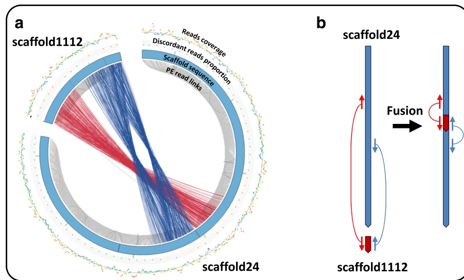
Fig. 3 Example of a clue leading to scaffold fusion. a Graphical representation of paired read leading to the identification of fusion of scaffold1112 into scaffold24. This representation is drawn using Scaffremodler's tools. In the inner circle, links between read pairs are drawn with the color code described in Fig. 2: grey for concordant pairs; red and orange for discordant in size; purple, green and blue for orientation discordant pairs. The second circle represents scaffold in blue with gaps as black regions. The next represents the proportion of discordant reads and the last circle represents read coverage as in Fig. 2. Red and blue beams linking scaffold1112 and scaffold24 allowed identifying scaffold fusion schematized in (b). Inserting scaffold1112 into scaffold24 will correct the discordant red links and correct the orientation of discordant blue links
