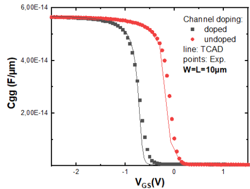
Fig. 2 : TCAD vs. Exp C_{GG} ( \text{F}/\mu\text{m} ) as a function of V_{GS} for both doped and undoped channel.
