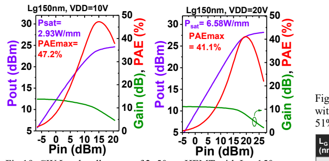
Fig.19: CW Load-pull sweep of 2x50 \mu m HEMT with L_G=150nm at 28 GHz. We obtain state of the art P_{OUT,MAX} of 2.9 W/mm at V_{DD}=10V and record 6.6W/mm at V_{DD}=20V for a CMOS compatible 200mm SiN/AIN/GaN/Si MIS-HEMT.
