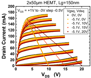
Fig.15: Pulsed-IV characteristics of a 2x50 \mu m HEMT with L_G=150nm . Each point of the I_D(V_{DS}, V_{GS}) curves is pulsed from a given stress bias point ( V_{gsq}, V_{dsq} ). G_L is negligible (light orange vs black curves) and DL is low up to 20V (dark red vs black curves). Straight lines are optimum load-lines for output power.
