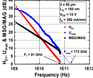
Fig.16: 2x50 \mu m HEMT H_{21} , U_{max} and MSG/MAG versus frequency. Extrapolation gives F_t/F_{MAX} = 81/173 GHz.
