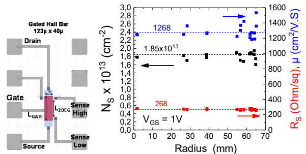
Fig.9: Extraction of low field channel parameters with a gated Hall bar structure (left). R S is measured with 4 points probe technique. N S is obtained by integration of C(V GS ) and μ = 1/(N S ·q·R S ) where q is the electronic charge. Uniformity across the wafer is shown in the right graph for V GS = +1V with median values of R S , N S and μ.
