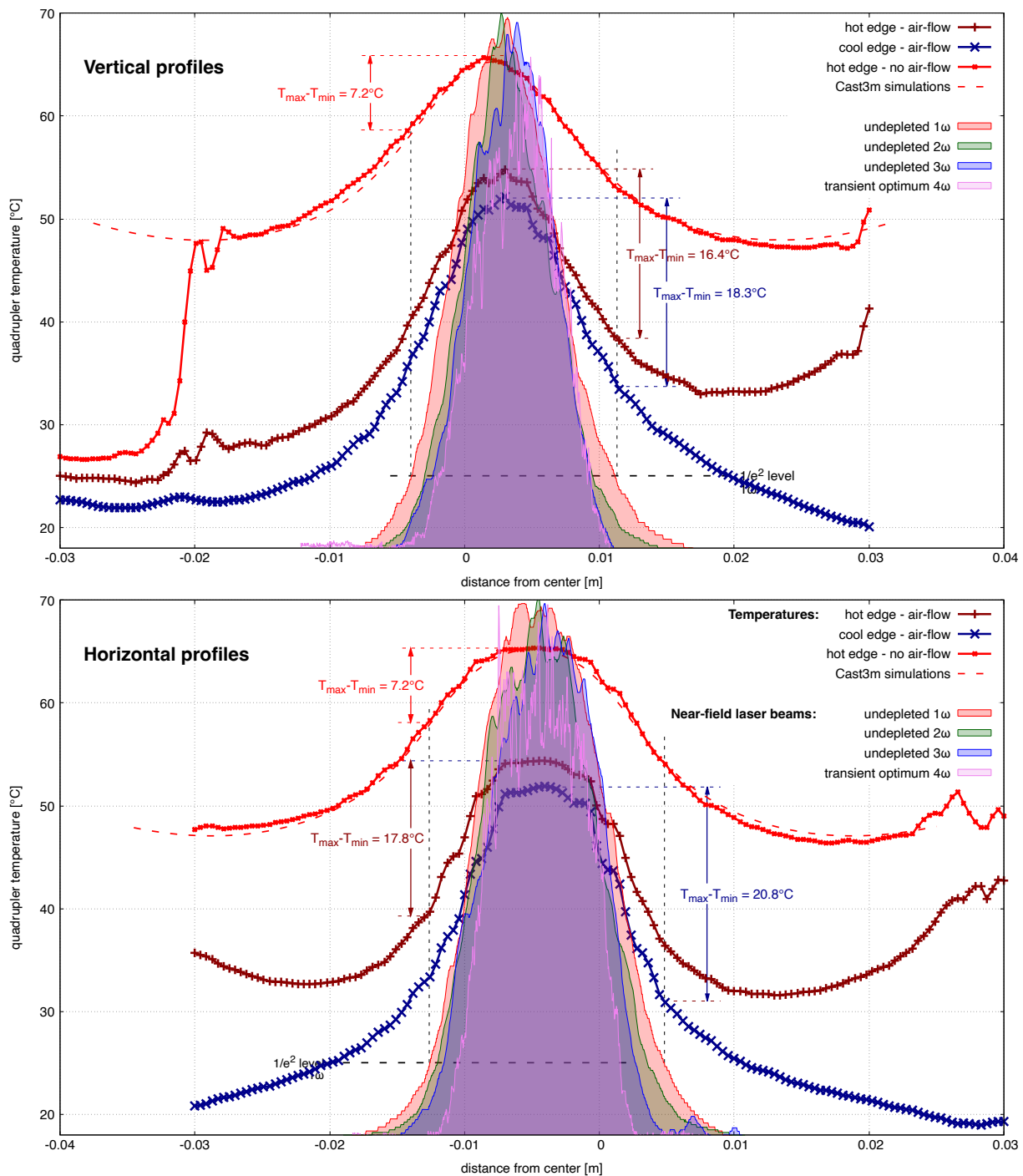
Figure 12. Measurements of temperature gradients in various conditions
