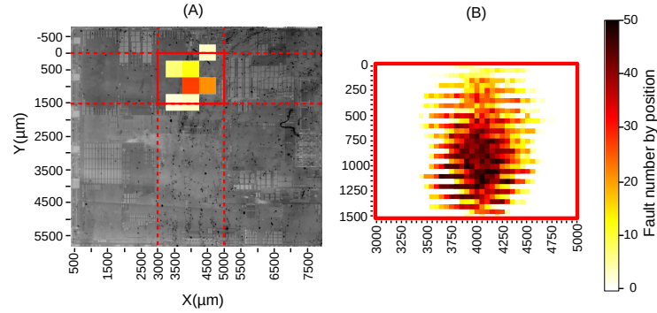
Fig. 4. Fault injection sensitivity scan for 400 V pulse.
