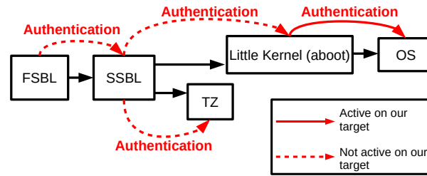
Fig. 5. Secure-Boot Architecture
