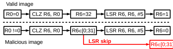
Fig. 7. Algorithm behavior
