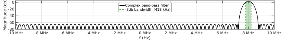
Fig. 3. Complex band-pass digital filter
