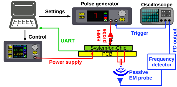
Fig. 9. Experimental setup
