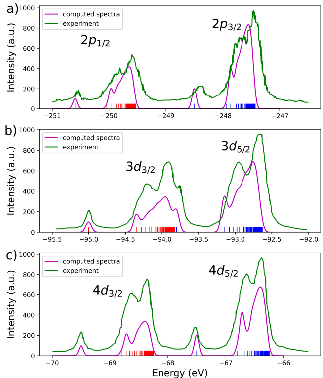
FIG. 3. Simulated and Experimental XPS spectra of a) Ar, b) Kr, and c) Xe cluster around 3000 atoms. Short vertical lines represent binding energy from each atom. A Gaussian broadening of 50meV was used.
