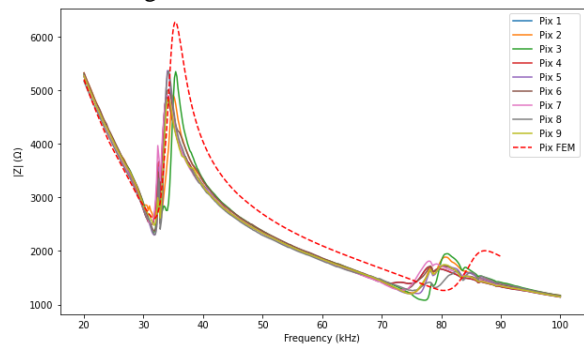
Figure 9: Impedance measurements for the nine pixels of the surface compared with the FEM.
