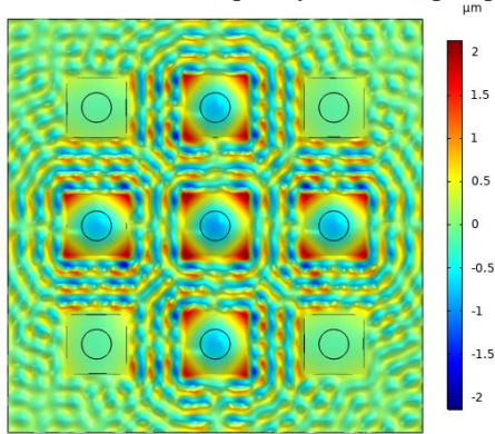
Figure 2 : « + » shape obtained from COMSOL model.
