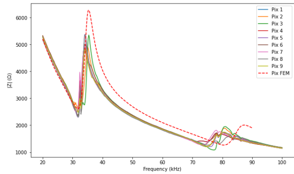
Figure 9: Impedance measurements for the nine pixels of the surface compared with the FEM.
