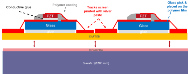
Figure 3: Schematic cross section of the interface fabrication process.
