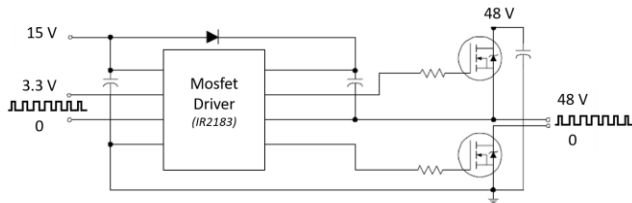
Figure 7: Amplification stage for one haptic pixel.
