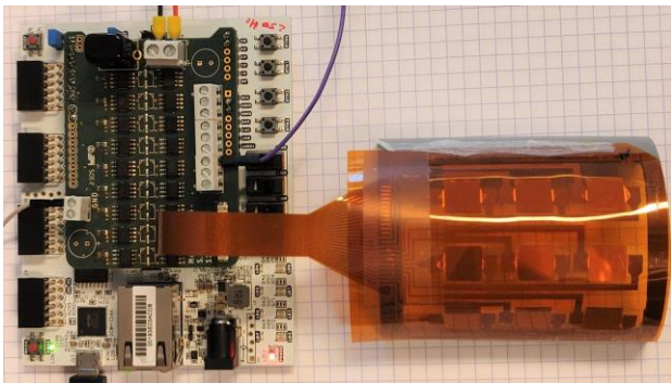
Figure 8: Actuation electronics with the interface on a cylindrical support.
