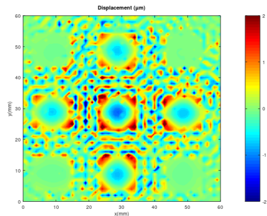
Figure 10: Laser vibrometer displacements measured for a "+" shape obtained with five actuated pixels.
