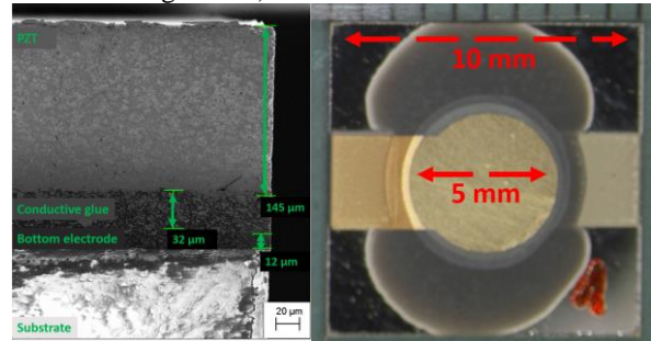
Figure 4: a) SEM cross section and b) top view of the haptic pixel.
