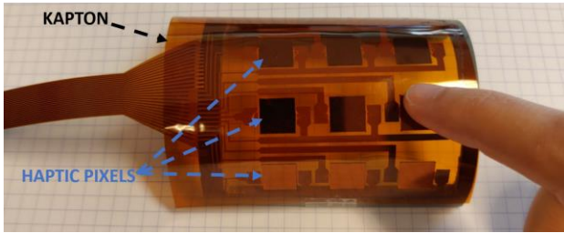
Figure 6: New flexible nine-pixel haptic interface.
