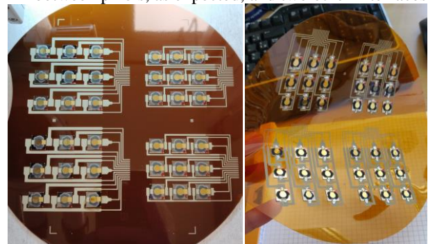
Figure 5: 4 haptic interfaces before and after the release of the REVALPHA from the silicon wafer.
