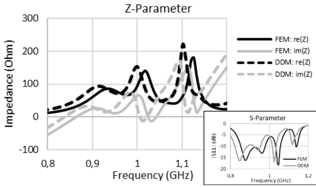
Fig. 6. Real and imaginary part of Z-parameter solved with FEM and DDM, and (inset) Magnitude of the reflection coefficient |S_{11}| , for a half-wave dipole over a finite mushroom-like AMC.
