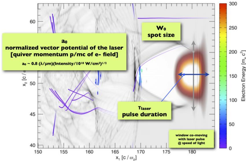
Figure 3.26. Schematic of laser wakefield acceleration. A strong laser pulse (depicted at the right of the simulation window in red) propagates in the plasma—the radiation pressure is strong enough to expel the electrons from the wakefield region, forming a bubble/electron cavity. The ions in the plasma column thus create an electric field that pulls electrons in, closing the bubble, but that also provides electron acceleration. Inside the bubble, electrons (coloured according to their energy) can accelerate and gain energy. Image courtesy of Samuel F Martins GoLP/IPFN/Instituto Superior Tecnico.
