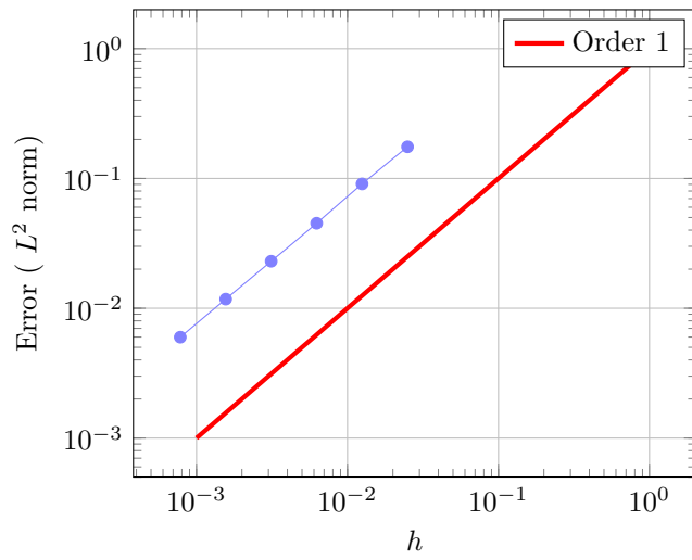
Figure 8 – Convergence curve for P_3 with the Glace scheme (Log scale). Top: random meshes, middle: Delaunay meshes, bottom: cartesian meshes.
