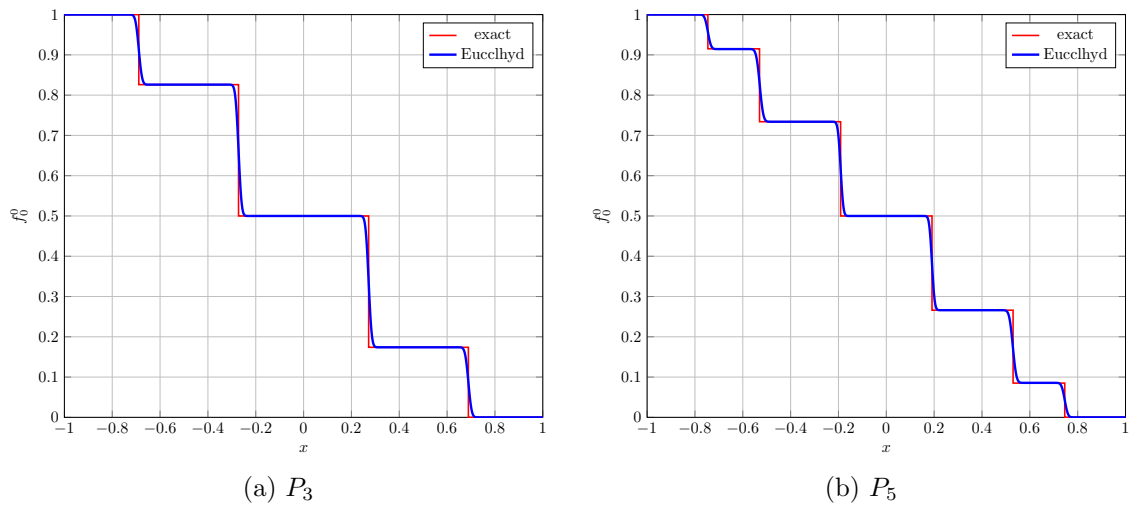
Figure 2 – Riemann problem with the Eucclhyd scheme on a cartesian mesh 3840 \times 4 at time t = 0.8 .
