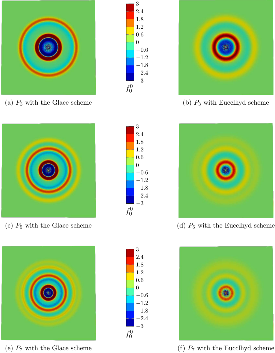
Figure 7 – Solution for a regularized Dirac type initial condition on a Delaunay mesh ( h = 3/320 ) at time t = 1 .
