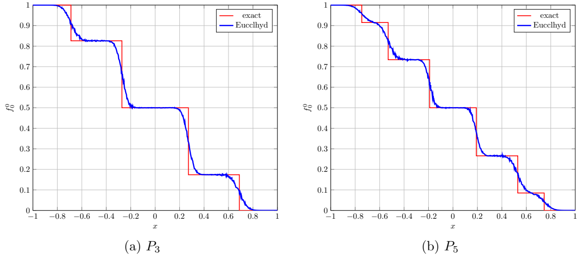
Figure 4 – Riemann problem with the Eucclhyd scheme, random meshes 320 \times 4 , t = 0.8 .
