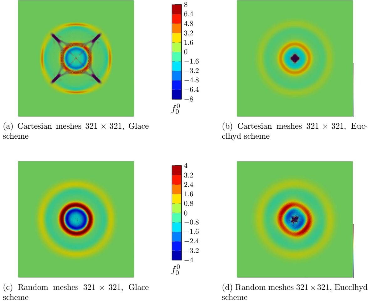
Figure 5 – Solution for a Dirac-like initial condition for P_3 at time t = 1 .
