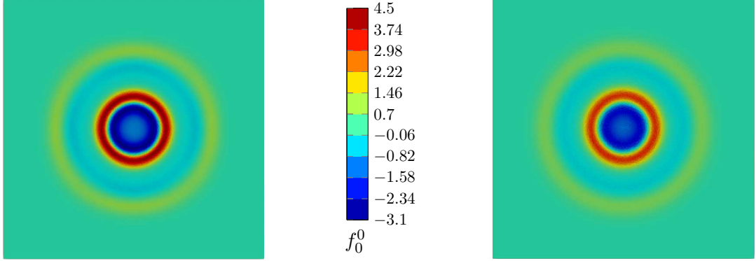
(a) P_3 on a random mesh 321 \times 321 with the Glace scheme
