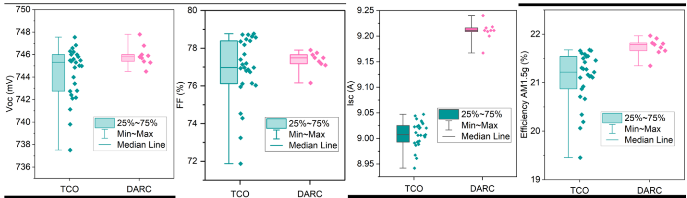
Figure 3 – V_{oc} , FF, I_{sc} & Efficiency under AM1.5g spectrum at room temperature for 60 \mu\text{m} p-type Ga-doped Si heterojunction solar cells, with single layer (TCO) and double layer (TCO + dielectrics) antireflection coatings.
