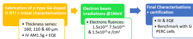
Figure 1 – Experimental plan for testing p-type Si Ga-doped heterojunction radiation hardness
