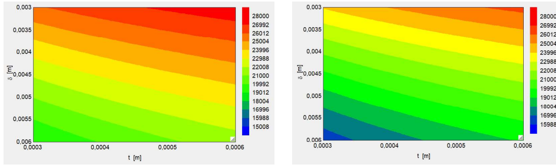
Figure 11: Effect of the spacing of the fins ( \delta ) and their thickness ( t ) on the withdrawal power (Watt) considering storage at 60°C and a flow rate of 700l/h (PEG6000 on the left and RT58 on the right)
