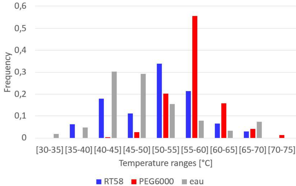
Figure 9: Average storage temperature (Nice)
