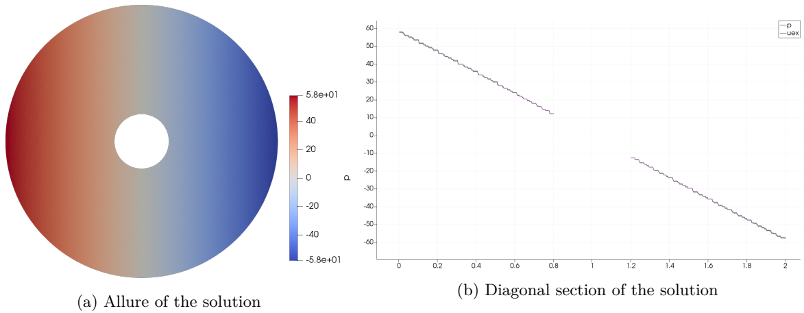
Figure 38: Solution (160) on an annulus mesh of triangles
