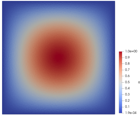
(a) Allure of the solution for \lambda = h^{\frac{1}{2}}
