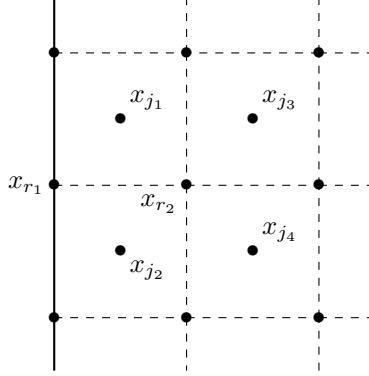
Figure 10: Structured mesh
