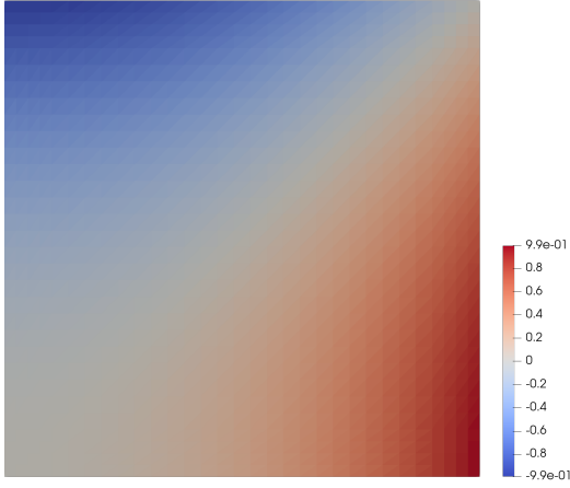
(a) Cell value on the left-sided triangle mesh - N = 80
