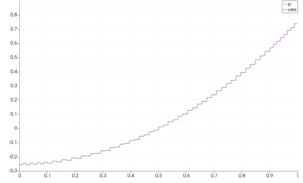
(b) Horizontal section on the left-sided triangle mesh
