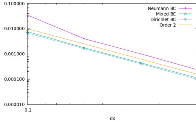
Figure 17: Convergence graph of the non linear unstationary solution (146) at T = 1
