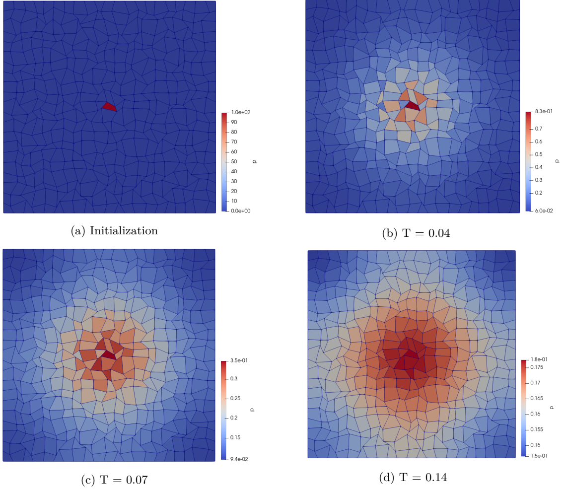
Figure 25: Spurious mode on a non-Cartesian mesh
