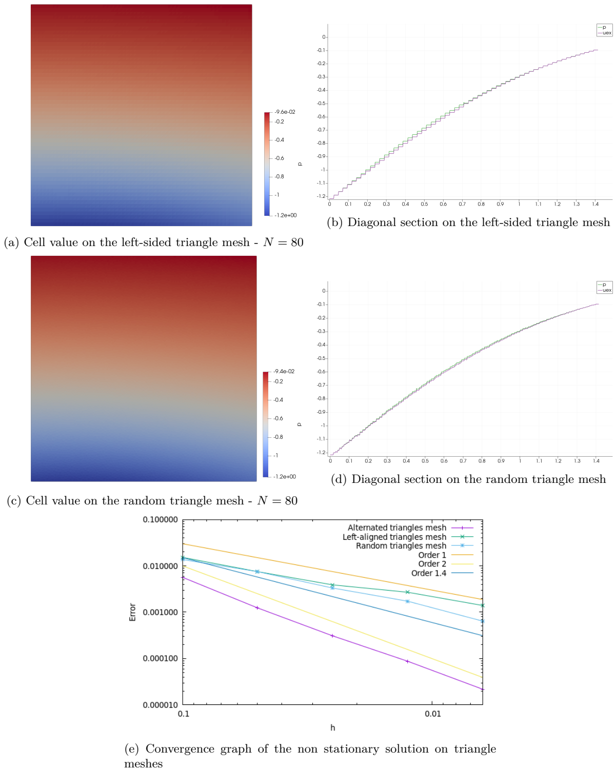
Figure 36: Allure of the solution (159) and its diagonal section at T = 10 with N = 80
