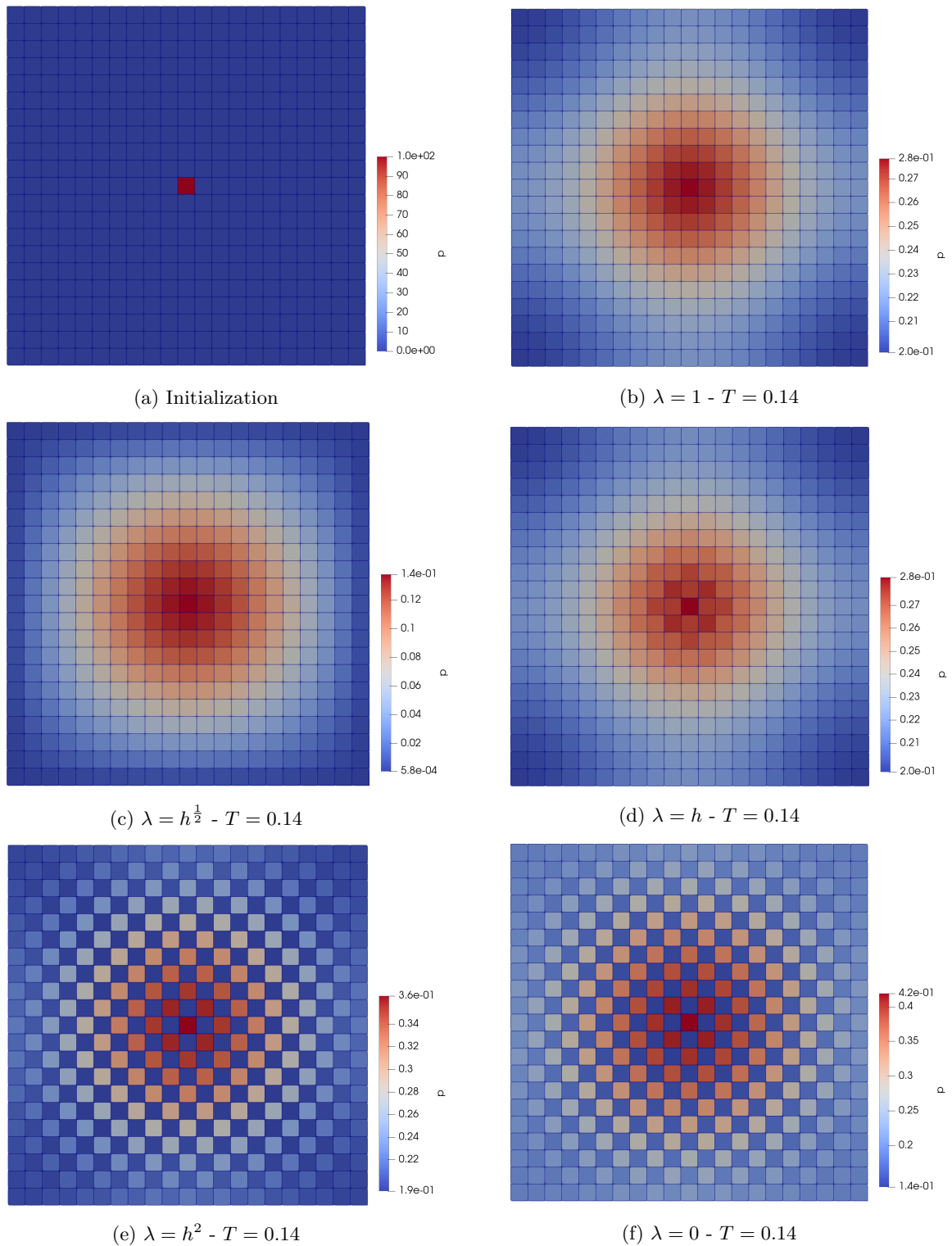
Figure 41: Spurious modes appearing depending the value of \lambda
