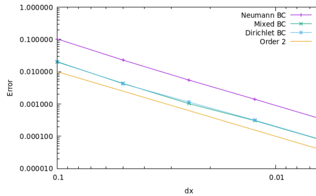
Figure 23: Convergence graph for the solution with a non constant \kappa (153)
