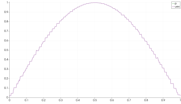
(b) Horizontal section of the solution for \lambda = h^{\frac{1}{2}}
