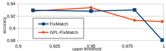
Fig. 2. Accuracy on the first fold of CIFAR-10-40 when the upper threshold varies. GPL makes the performance more robust with respect to the upper threshold.
