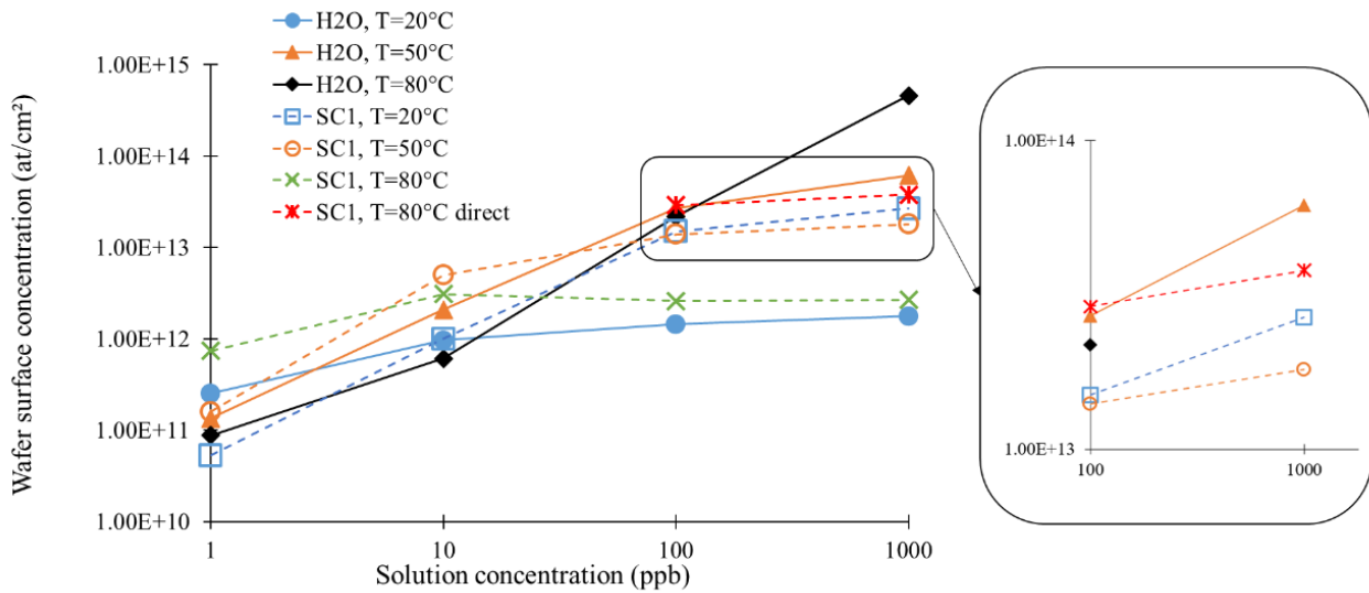
Figure 5. Surface concentration of iron determined by TXRF as a function of the level of contamination added to the SC1 bath 1:1:5 and the H 2 O bath for different temperatures, treatment time of wafers in the bath is 5 min.
