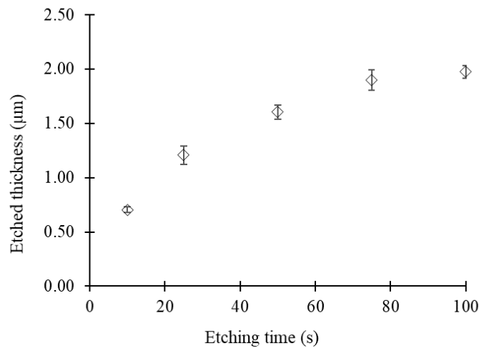
Figure 4. Etch rate for LPD-Bulk, calculated from the weight of the wafer.
