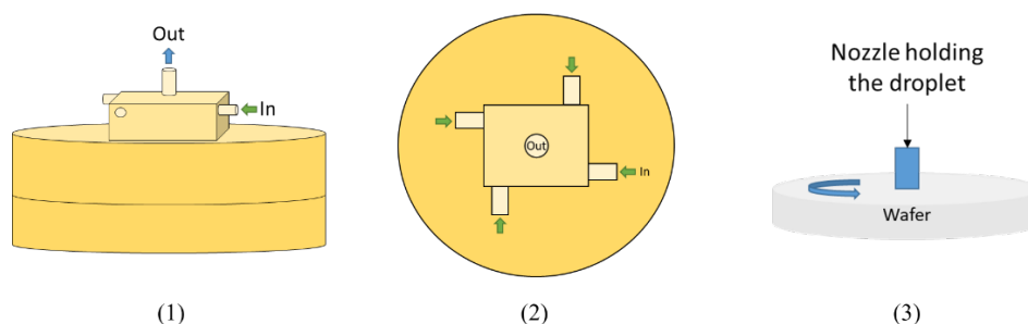
Figure 1. (1) VPD chamber side-view, (2) VPD chamber viewed from above, (3) collection of contaminants by a HF/H 2 O 2 droplet.
