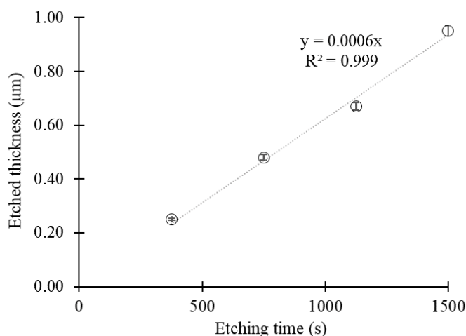
Figure 2. Etch rate for VPD-Bulk, measured by model-based infrared spectroscopy.
