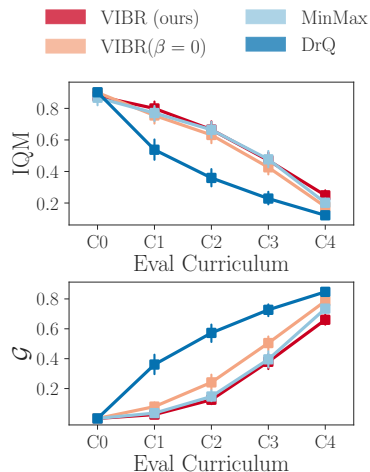
Figure 4: Evaluation score over ablations and variations of VIBR. Shaded areas are bootstrapped CI.
