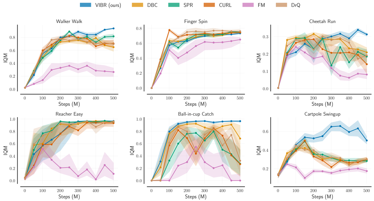
Figure 9: Evaluation sample efficiency curves on C1. Line IQM and shaded area bootstrapped CI.
