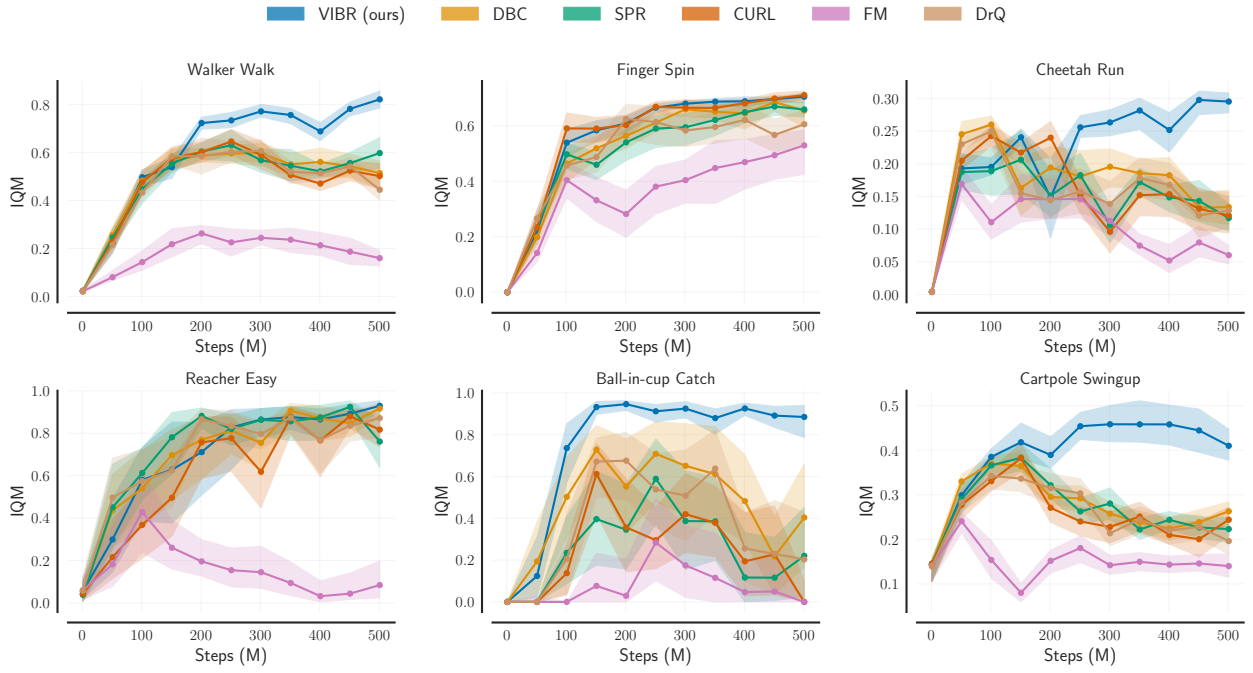
Figure 10: Evaluation sample efficiency curves on C2. Line IQM and shaded area bootstrapped CI.
