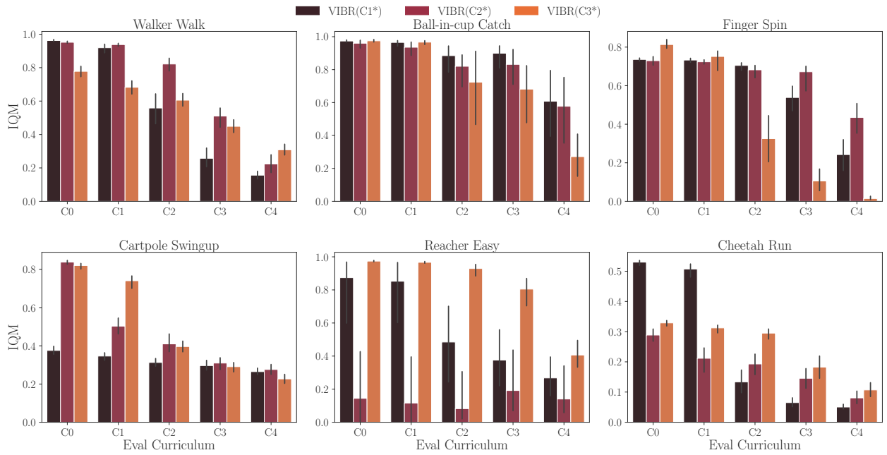
Figure 15: IQM per environment per evaluation domain while changing training domain. Vertical bars are bootstrapped CI.
