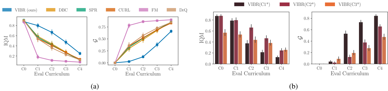
Figure 3: (a) : Evaluation score (IQM and Generalization Gap) of VIBR and baselines over all 5 evaluation domains. Vertical bars are bootstrapped CI. (b) : Effect of training curriculum on generalization.
