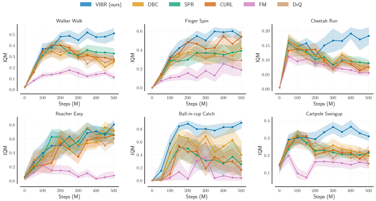
Figure 11: Evaluation sample efficiency curves on C3. Line IQM and shaded area bootstrapped CI.
