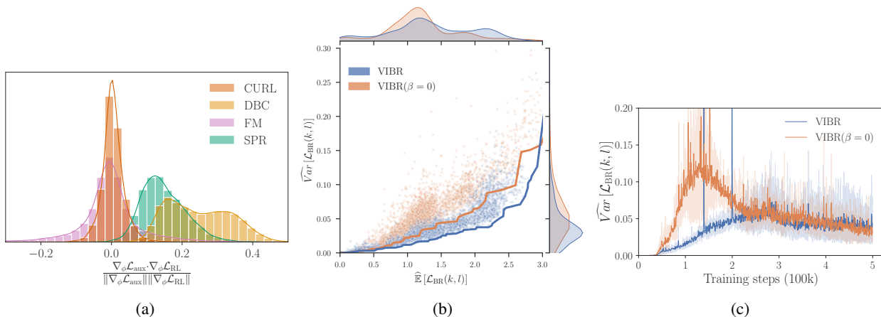
Figure 5: (a) : Cosine similarity between RL and auxiliary task during training of representation learning baselines. (b) : Distribution and lower Pareto frontier of VIBR loss components during training over 4 seeds. (c) : Evolution of empirical inter-observer variance loss during training.
