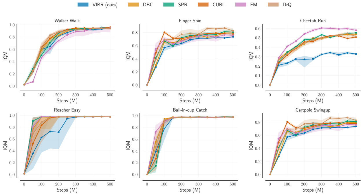
Figure 8: Evaluation sample efficiency curves on C0. Line IQM and shaded area bootstrapped CI.
