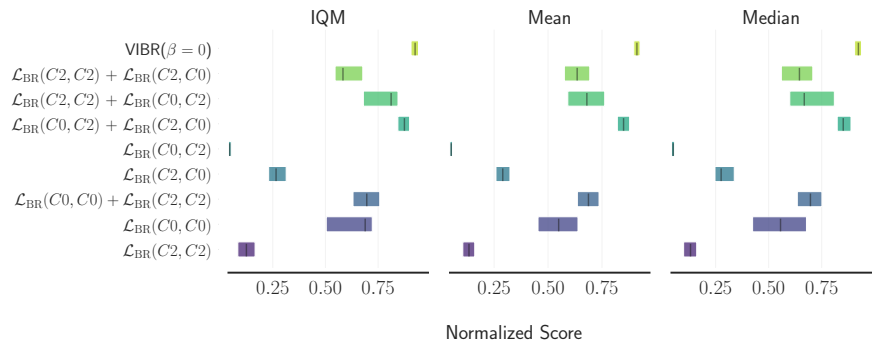
Figure 18: IQM and bootstrapped CI of ablations on C1
