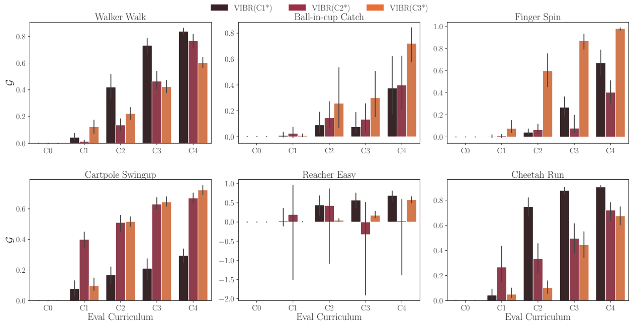
Figure 16: Generalization Gap per environment per evaluation domain while changing training domain. Vertical bars are bootstrapped CI.
