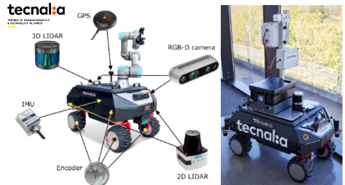
Fig. 9. (Left) RB-VOGUI (Robotnik), and sensors used by Tecnalìa to achieve autonomous navigation and localization of the platform. The platform's dimensions are 104 cm × 65 cm × 56 cm.
