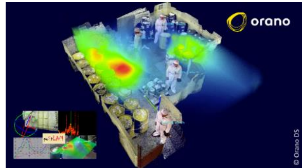
Fig. 11. Overlay and avatar positioning in a 3D reconstructed scene in PoStLAM (ORANO).
