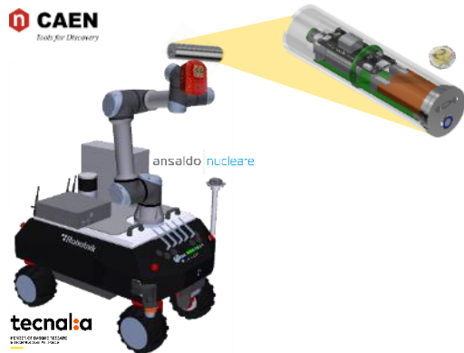
Fig. 7. Preliminary mounting configuration of the compact CZT sensor (CAEN) and Nanopix (CEA List) on the UR 5e robotic arm (Universal Robots).
