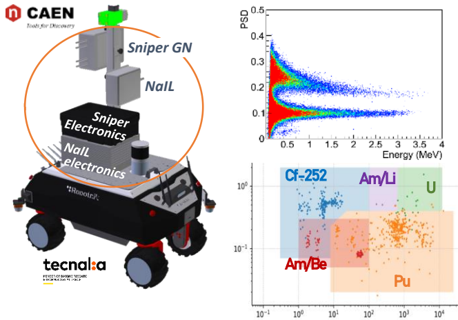
Fig. 6. CAEN's Sniper GN (CeBr 3 and stilbene scintillators) and Gamon (NaIL™ scintillator) mounted on the UGV (left) and example of gamma pulse-shape discrimination (top right). The latter, in combination with neutron measurement, enables to identify Nuclear Materials (bottom right) even when hidden behind gamma or neutron shielding.
