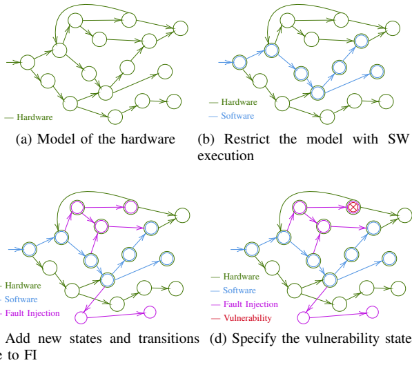
Figure 5: Modeling steps for FI vulnerability evaluation. fault model, the targeted signals are no longer under the control of the fault model.
