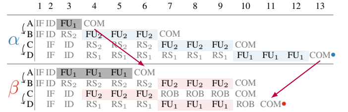
Figure 3: Execution traces showing the assignment to functional units (FU) and a reversal of the order of commits (red arrow) representing a counter-intuitive TA, obtained from the OoO template and the program of Fig. 2 (with superscal = 2 and N_{FU} = 2 ) [6].
