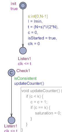
Fig. 4. UPPAAL transitions.
