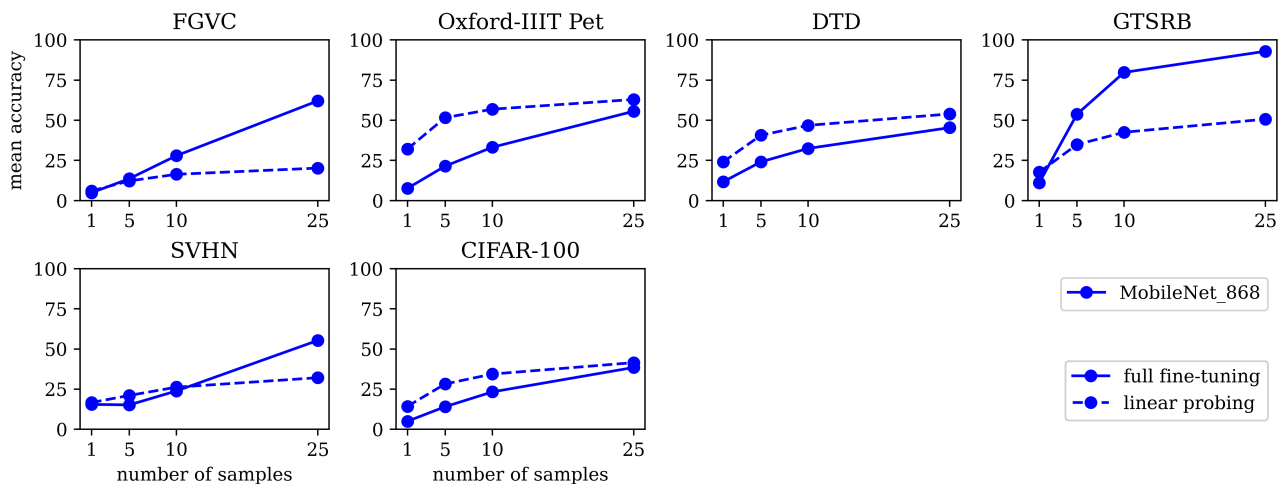
Figure 7: Downstream accuracy for each downstream task with 1000 classes and 500 images per classes for the pre-training.
