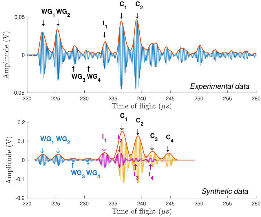
Figure 2: Top: experimental time series of the received signal when the silicon is fully liquid and the distance between the tip of the waveguide and the crucible is set to e_{l_0} = 21 mm. Echoes WG_1 to WG_4 are back reflections inside the waveguide. The echo I_1 is interpreted as the reflection at the crucible surface. Echoes labelled C_1 and C_2 corresponds to the reflections on the bottom of the crucible after crossing the 5 mm of graphite thickness. Bottom: synthetic data with calculated times of flight highlighting that echo I_2 is hidden by the echo C_1 in the experimental data (see text for details). Red curves are the envelopes of the signals.
