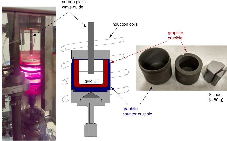
Figure 1: Left: photograph of the apparatus: the Beatrice furnace contains a melted silicon load; a silicon drop still hangs at the tip of the waveguide that has been dipped into the melt during several dozens of minutes before being removed. Middle: scaled illustration of the furnace in which the waveguide (dark grey rectangle), the graphite crucible (red) and the counter-crucible (blue) are represented. Right: the silicon load, the graphite crucible and the counter-crucible.
