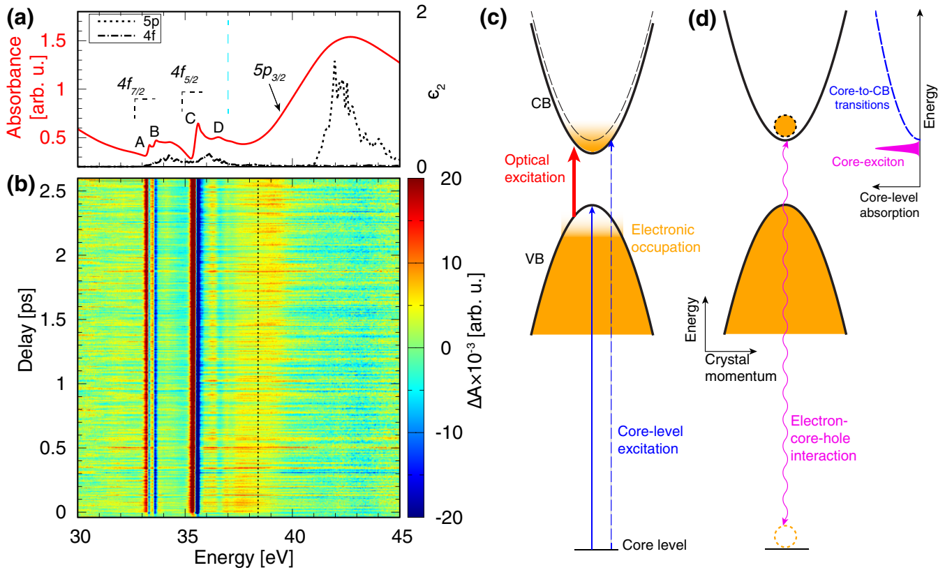
FIG. 1. (a) Static core-level absorption spectrum of a 40-nm-thick WS 2 film (red line). The dashed and dash-dotted black lines show the computed imaginary part of the dielectric function \epsilon_2(\omega) from the 5p and 4f core bands, respectively. (b) exhibits the XUV TA spectra between -40 fs and 2.6 ps delay. To serve as a reference (see text), a dashed cyan line is plotted at 37 eV in (a), and a dashed black line is plotted at 38.4 eV in (b). The scheme for a typical core-level TA measurement in highly screened semiconductors is shown in (c), where the core-level excitation probes the electronic occupation in the VB and CB plus the energy shift of the bands. (d) illustrates the formation of the core exciton through electron-core-hole attraction and its corresponding absorption spectrum.
