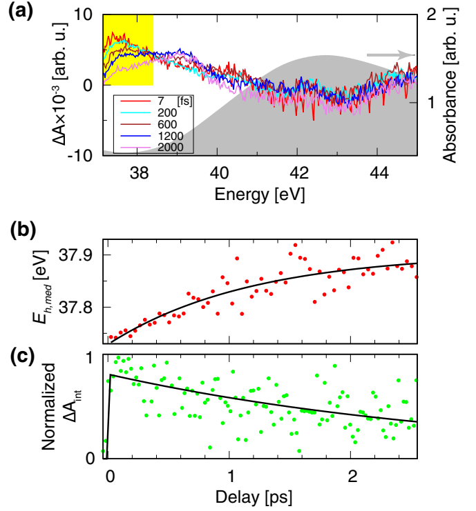
FIG. 3. (a) XUV TA spectra at the W O_3 edge at five different time delays. The static core-level absorption spectrum is plotted in gray as a reference. (b) shows the median energy E_{h,med} of the TA signal between 37.4 and 38.4 eV [yellow shaded area in (a)], and (c) shows the integrated XUV TA signal in the same energy region.
