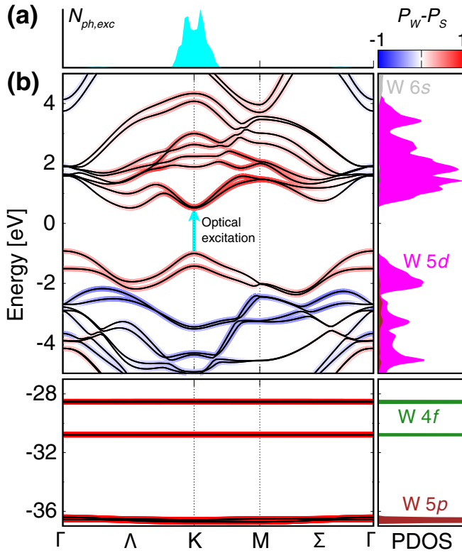
FIG. 4. (a) Number of photons in the optical pulse available to excite carriers from the VB to the CB as a function of k points (Appendix C). (b) shows the band structure and projected density of states (PDOS) of WS_2 calculated with the FP-LAPW method (Appendix C). The colors on the bands (left panel) reflect the difference between the atomic orbital projection on W and S ( P_W - P_S ). P_n is the sum of the modulus square of the wave-function projections of atom n .
