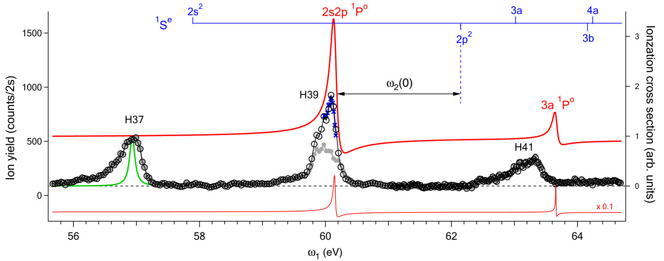
FIG. 2. Measured ion yield (empty black circles) as a function of the monochromator pass energy covering the H37 – 41 wavelength region with the coupling laser off. Thick (red) curve is the theoretical helium photoabsorption cross section [16], convoluted by a 100 meV FWHM Lorentzian (thick green curve) and scaled to 1 on the top of H37 . Thin (red) curve denotes the shape of the unconvoluted cross section. The ratio of the measured ion signal (with background subtracted) and the convoluted cross section (full gray circles) estimates the ion yield signal for a fictitious case with no 2s2p\ ^1P^o resonance. The top bar gives energy positions of the lowest-lying 1S^e resonances with dashed line showing the position of the 2p^2\ ^1S^e state. The ion yield signal observed in the limited range of the ATS measurement with a strongly delayed EUV pulse [Fig. 4(a)] is denoted by (blue) crosses.
