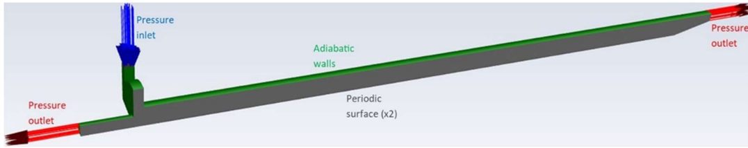
Fig. 3 Boundary conditions
