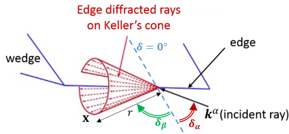
Fig. 2: Keller's cone of diffraction
