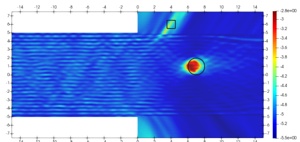
Figure 1: Level curves of the imaging function \mathbf{z} \mapsto -\log(\|h^{reg}(\mathbf{z})\|_{L^2(\Sigma_{-R})}) for two Dirichlet obstacles in a steel plate partially buried in concrete, using 26 propagating modes. Parameters: h = 5 , h_{in} = 7.5 , h_{out} = 12.5 , 10% of noise.
